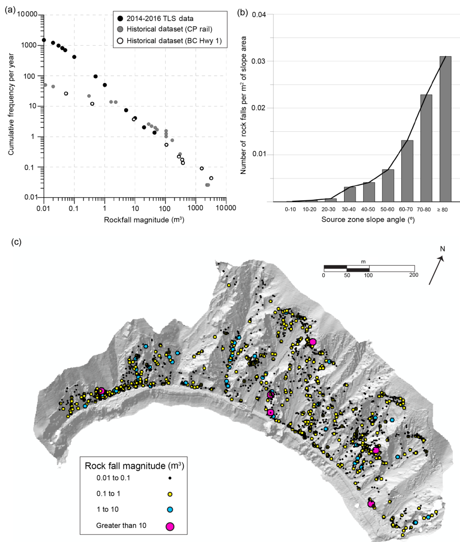
Figure 5. (a) Magnitude–cumulative–frequency curves for rockfalls extracted from TLS compared to historical records (digitized from Hungr et al., 1999). (b) Graph of rockfall frequencies based on source zone slope angles. (c) Spatial distribution of rockfall event locations from TLS data collected between 11 November 2014 and 2 May 2016.
