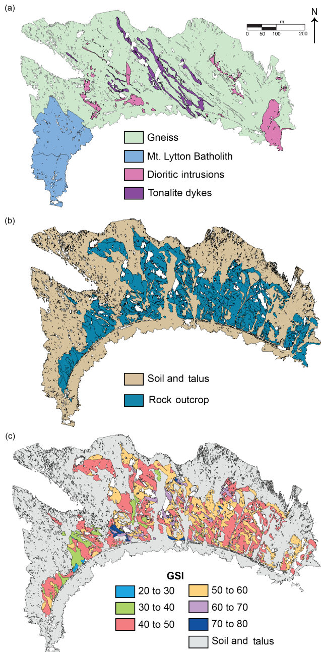
Figure 4. Classified slope models for White Canyon West based on: (a) lithology; (b) ground cover type and (c) GSI. White spaces represent oclusions in the model.
