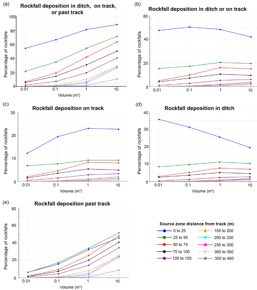
Figure 9. Rockfall deposition percentages based on classified outputs from the RockyFor3D model showing (a) percentage of rockfalls deposited in the ditch, on tracks, or past the tracks, (b) in the ditch or on the tracks, (c) on the tracks, (d) in the ditch and (e) past the tracks (on the downslope side).
