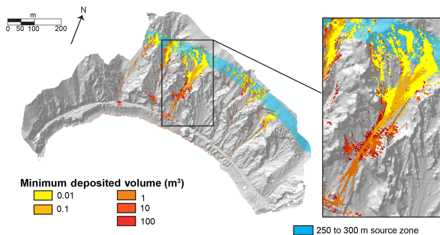
Figure 8. Example of deposition outputs from the RockyFor3D model for the 250 to 300 m source zone. Coloured cells indicate rockfall deposition points and the colour of the cell represents the minimum volume deposited in each cell: for example, the darkest red colour represents cells in which only blocks 100 m 3 were deposited, and the second darkest colour represents cells in which blocks 10 m 3 or larger (100 m 3 were deposited).
