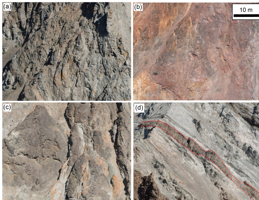
Figure 3. Examples of the four main geological units in the White Canyon. (a) Quartzofeldspathic gneiss (Lytton Gneiss); (b) red-stained granodiorite (Mt. Lytton Batholith); (c) dioritic intrusions and (d) tonalite dyke (outlined in red).
