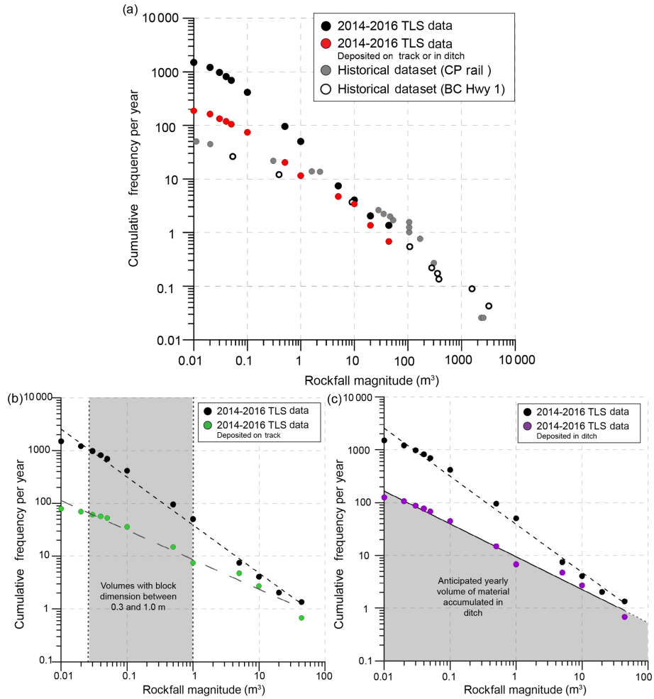
Figure 10. (a) Modified MCF curves for rockfalls deposited on track or in the ditch compared to TLS inventory and historical data, (b) modified MCF curves for rockfalls deposited on track compared to TLS inventory and (c) modified MCF curves for rockfalls deposited in the ditch compared to TLS inventory.
