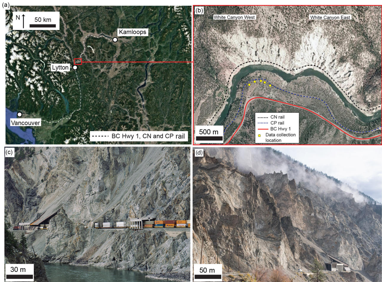
Figure 1. (a) Location of the White Canyon. (b) Plan view of the White Canyon West and East slopes with the location of highway and rail lines indicated. Panels (c) and (d) Photographs of the White Canyon West illustrating complex geometry formed by deeply incised talus channels and vertical outcrops. Rock sheds are located at the base of several talus channels to guide material over the railway tracks.
