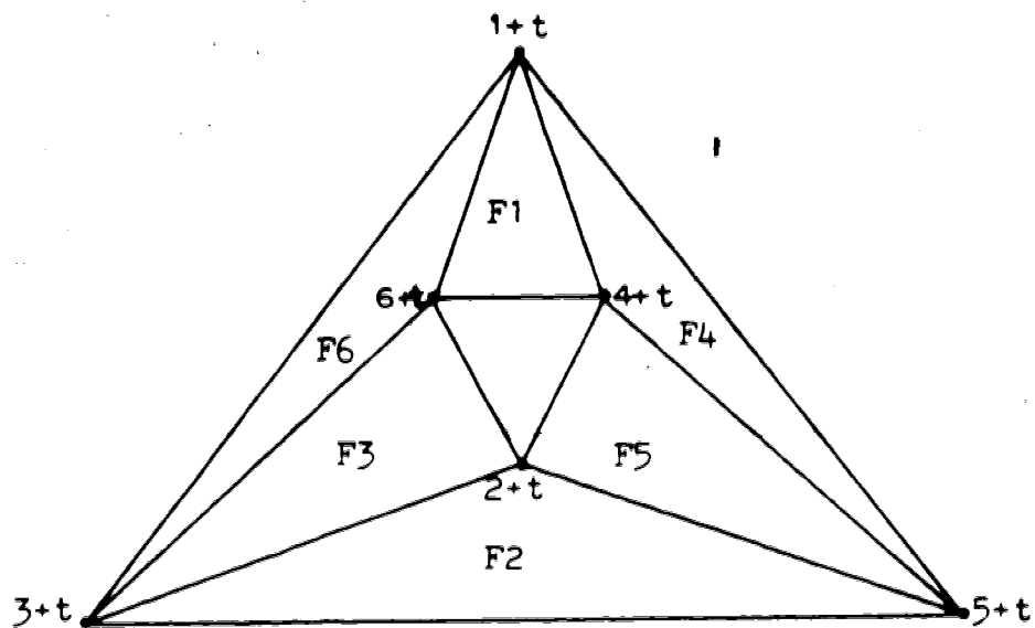
(a) The General Form of H_r
