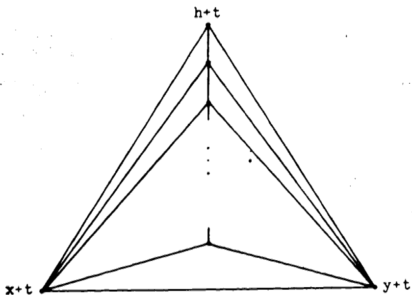
(a) The General Form of H_r
