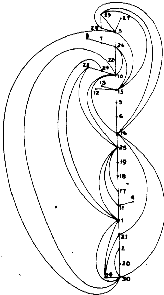
(c) H2 of G(30, 1, 5)
