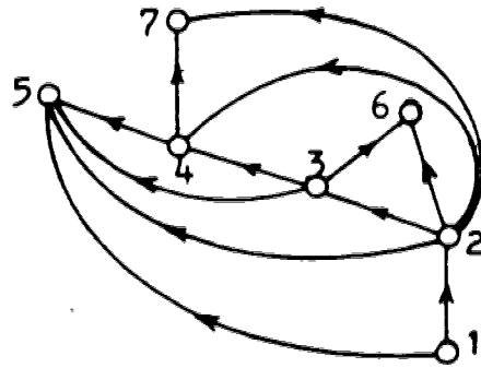
(a) The graph G
