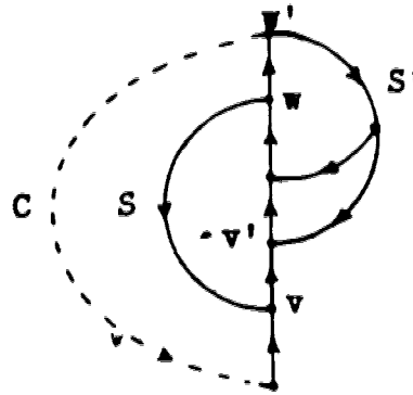
(a) v, v', w, w'
