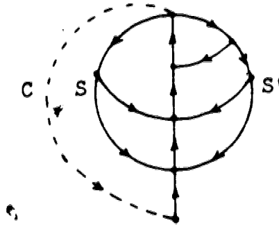
(b) Three common vertices
