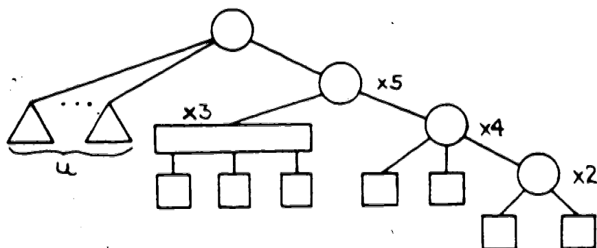
(d) Tk' after x_1 is deleted from Tk
