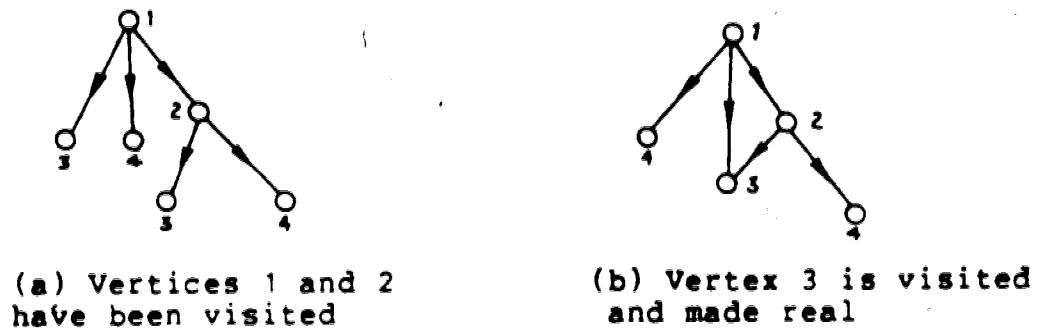
Figure 15. Real and Virtual Vertices
