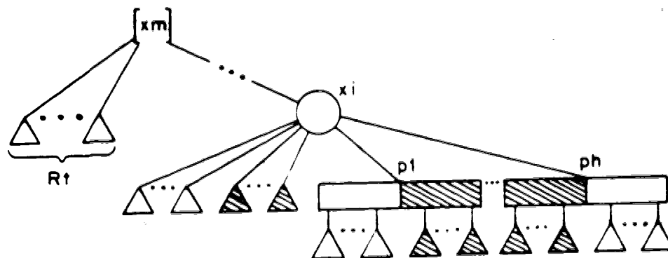
Figure 25. The Form of an Unmatched p-node
