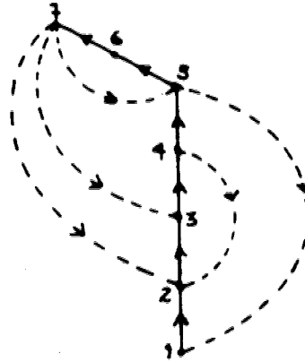
(a) The graph G.
