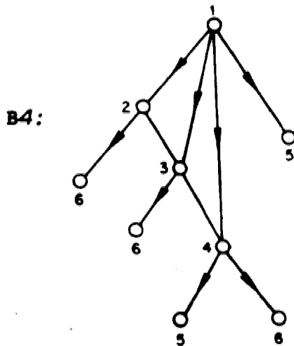
Figure 16. Embeddings and the Corresponding pq-trees
