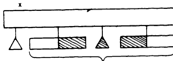
(b) A qdp-group of a q-node x
