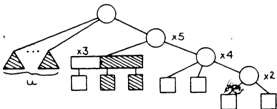
(e) The tree prior to x_5 being visited
