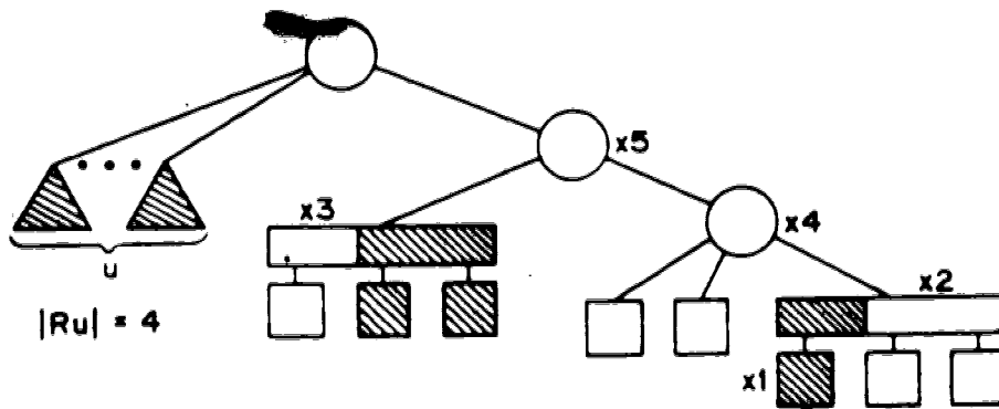
(a) Tk() before x_4 is visited
