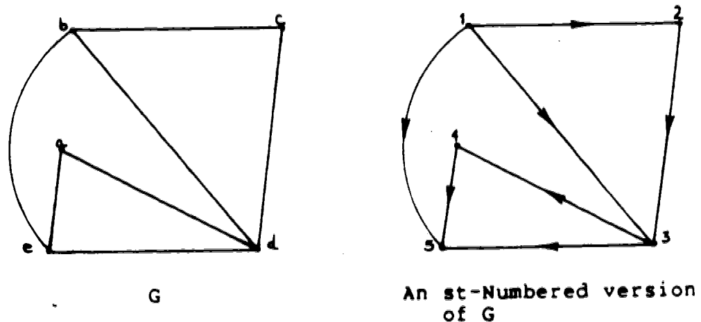
Figure 14. An st-numbering of a Graph
