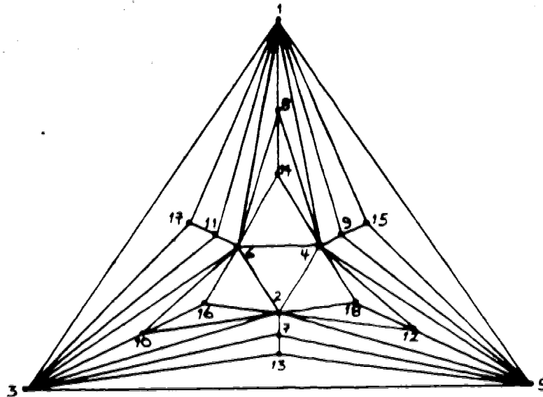
Figure 3. The subgraph H_1 of K_{18}
