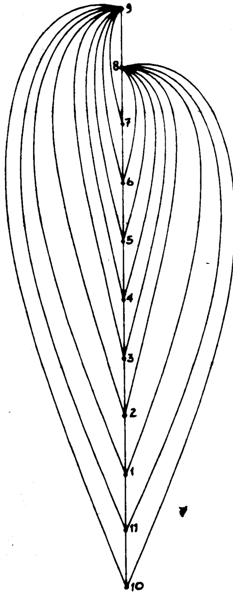
(a) H_1 of K_{11}
