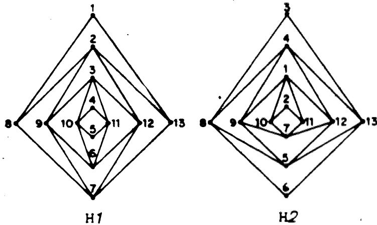
Figure 1. A Planar Partition of K(6,7)
