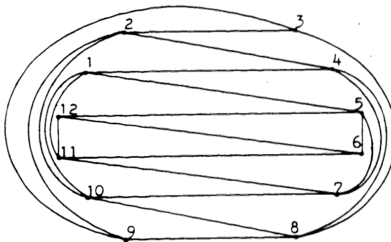
(b) The subgraph H_2 of K_{12}
