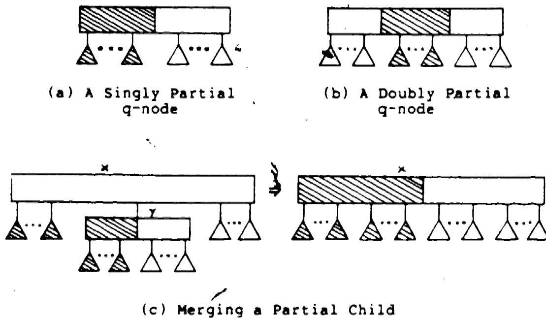
Figure 24. The Form of q-nodes in a pq-tree
