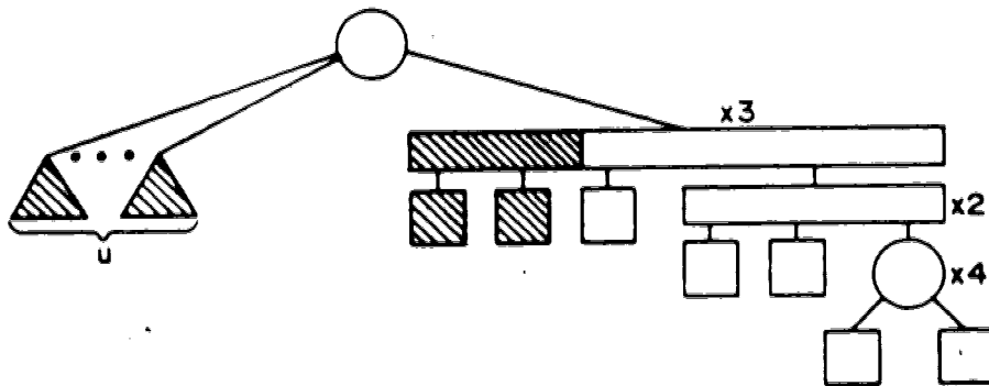
(c) After the deletion of x_1 and the reduction of x_5
