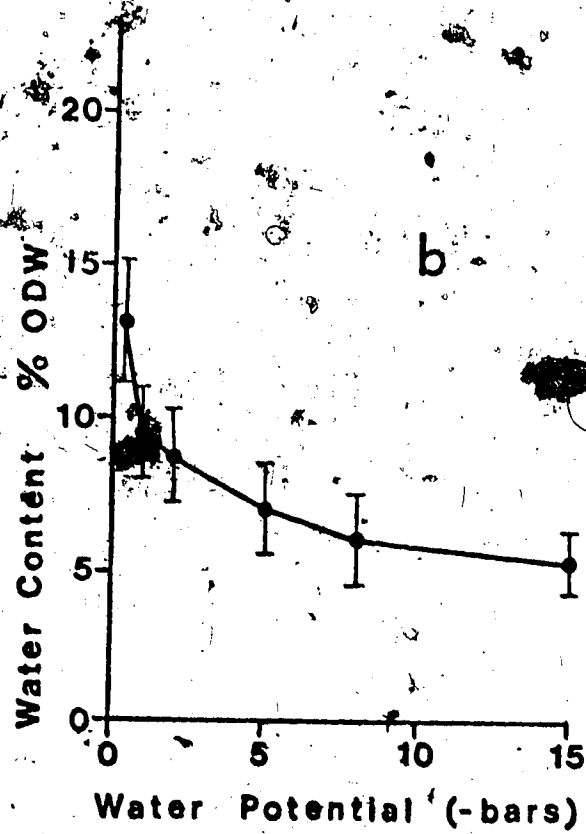
Figure 15. Water retention curves for soils (0-5 cm) from the Moss-Lichen-Rush (a) and Lichen-Moss-Rush (b) communities. Means \pm 95% confidence limits.
