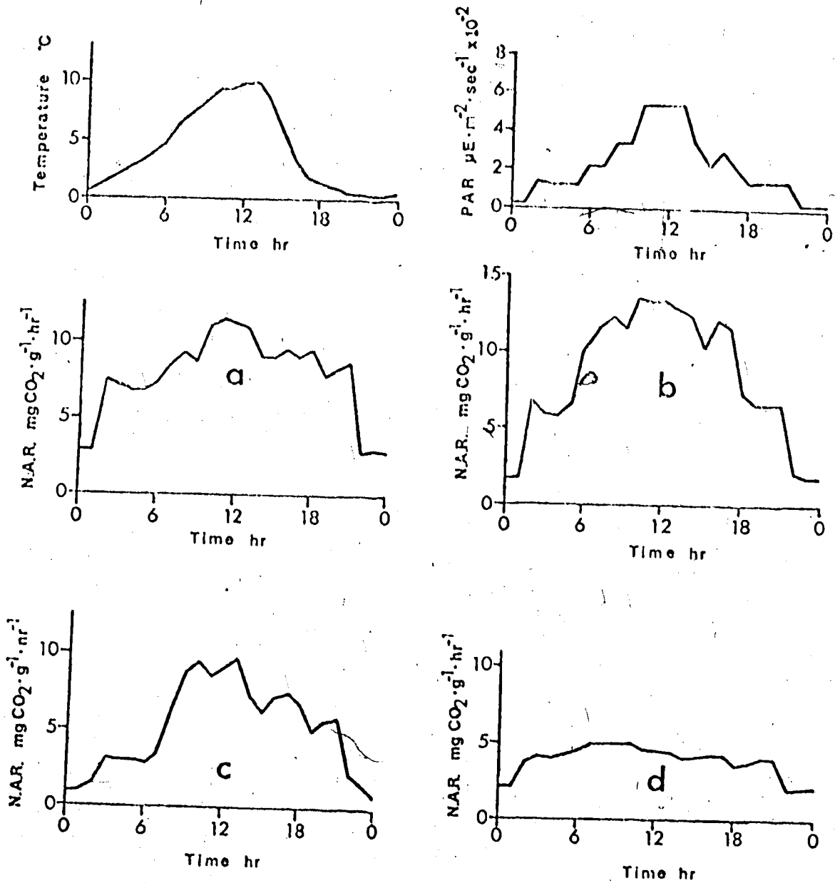
Figure 29. Net assimilation rate of Luzula confusa under four phenological stages in the laboratory; (a) preflowering, (b) anthesis, (c) postflowering and (d) dieback.
