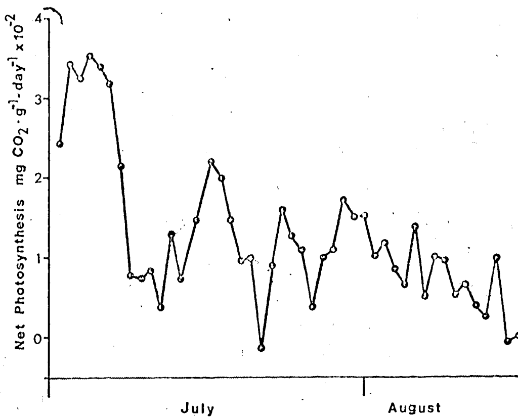
Figure 32. Potential net photosynthetic rate (field model) based on actual field conditions during the summer of 1973.
