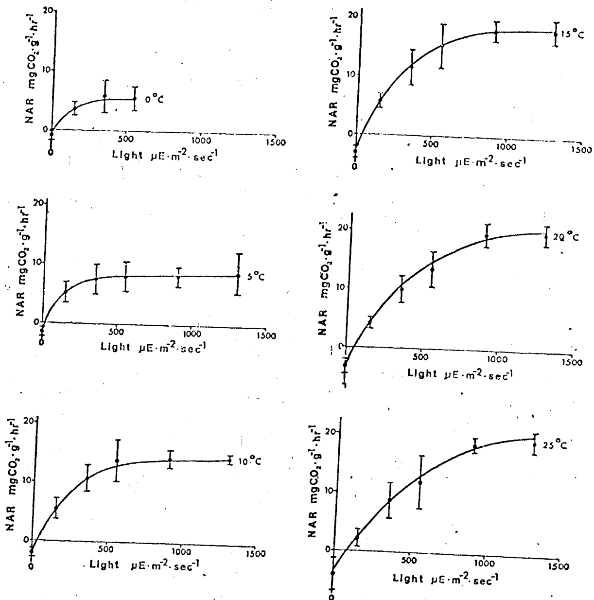
Figure 26. Net photosynthetic light response curves at various temperatures for Luzula confusa . All points are means with 95% confidence limits. Values are of 9-11 tillers from 8 different plants.
