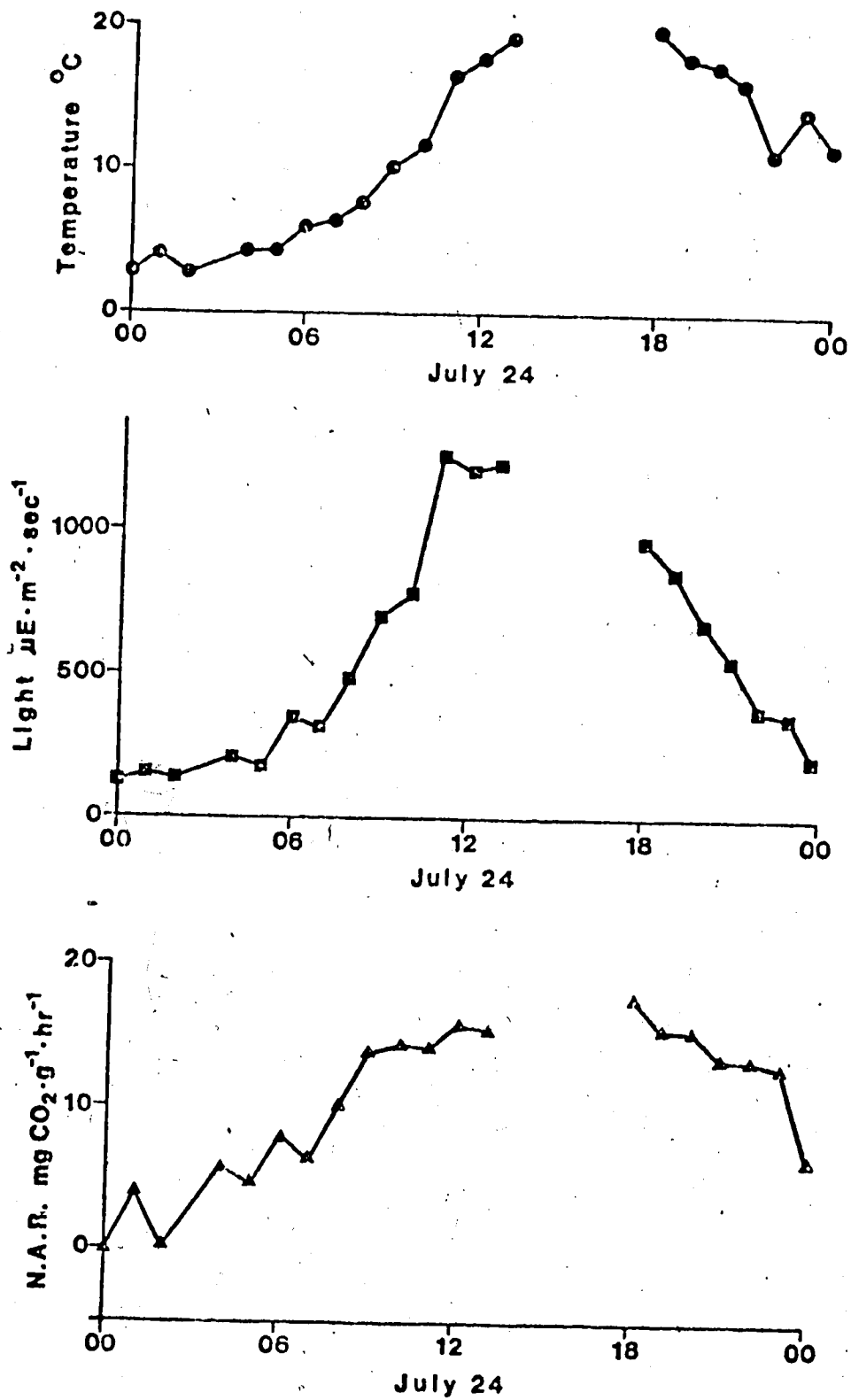
Figure 24. Net assimilation rate of Luzula confusa and environmental conditions during July 24, 1975.
