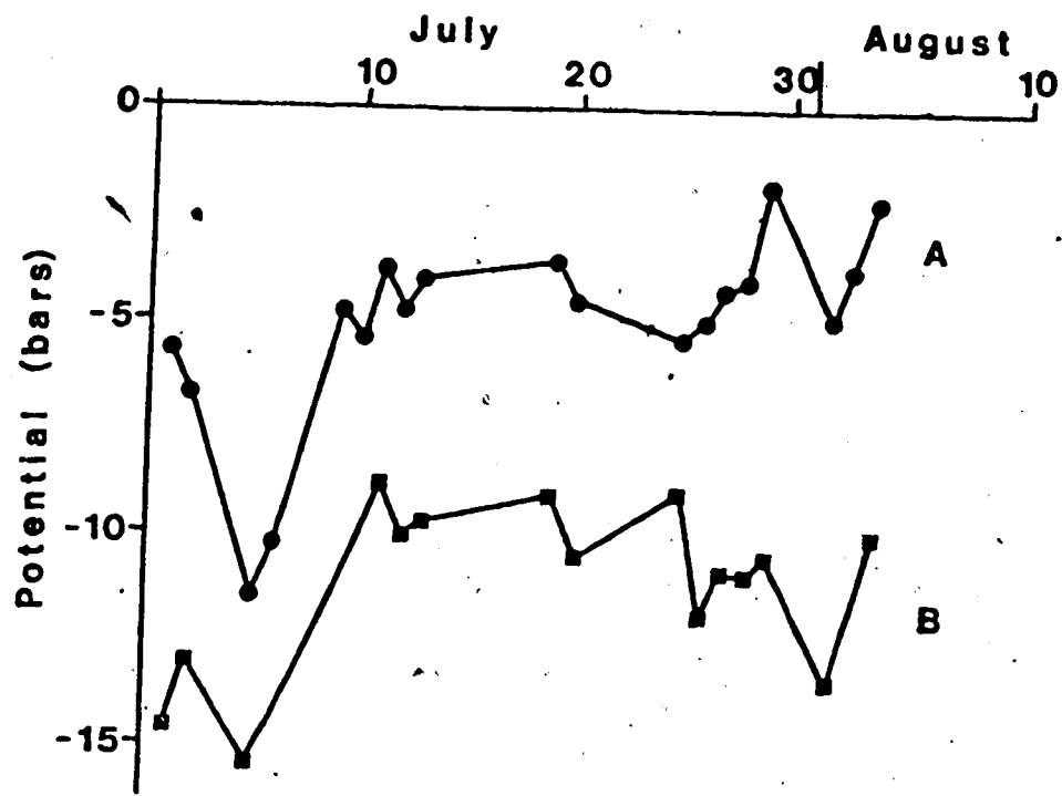
Figure 18. Leaf water potential (a) and osmotic plus matric potential (b) of Luzula confusa during the summer of 1974
