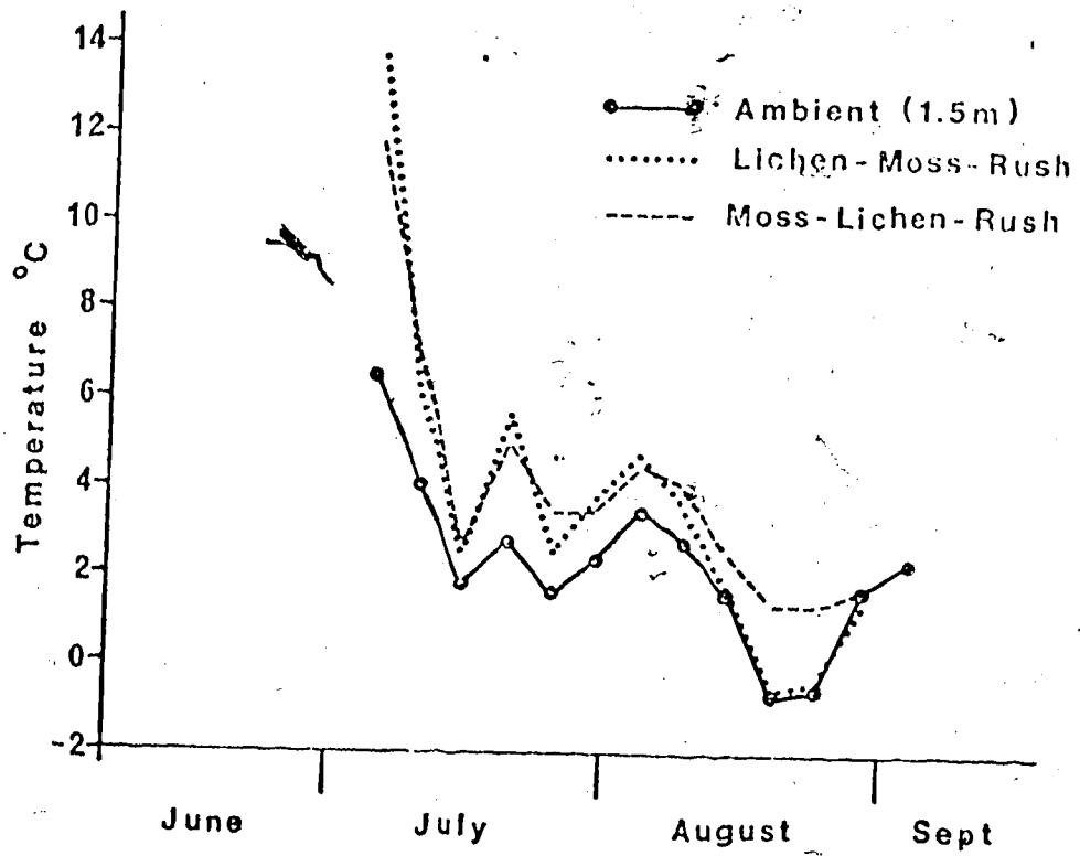
Figure 6. Temperature at 1.5 m and surface of the two plant communities during the summer of 1973. Values are weekly means.
