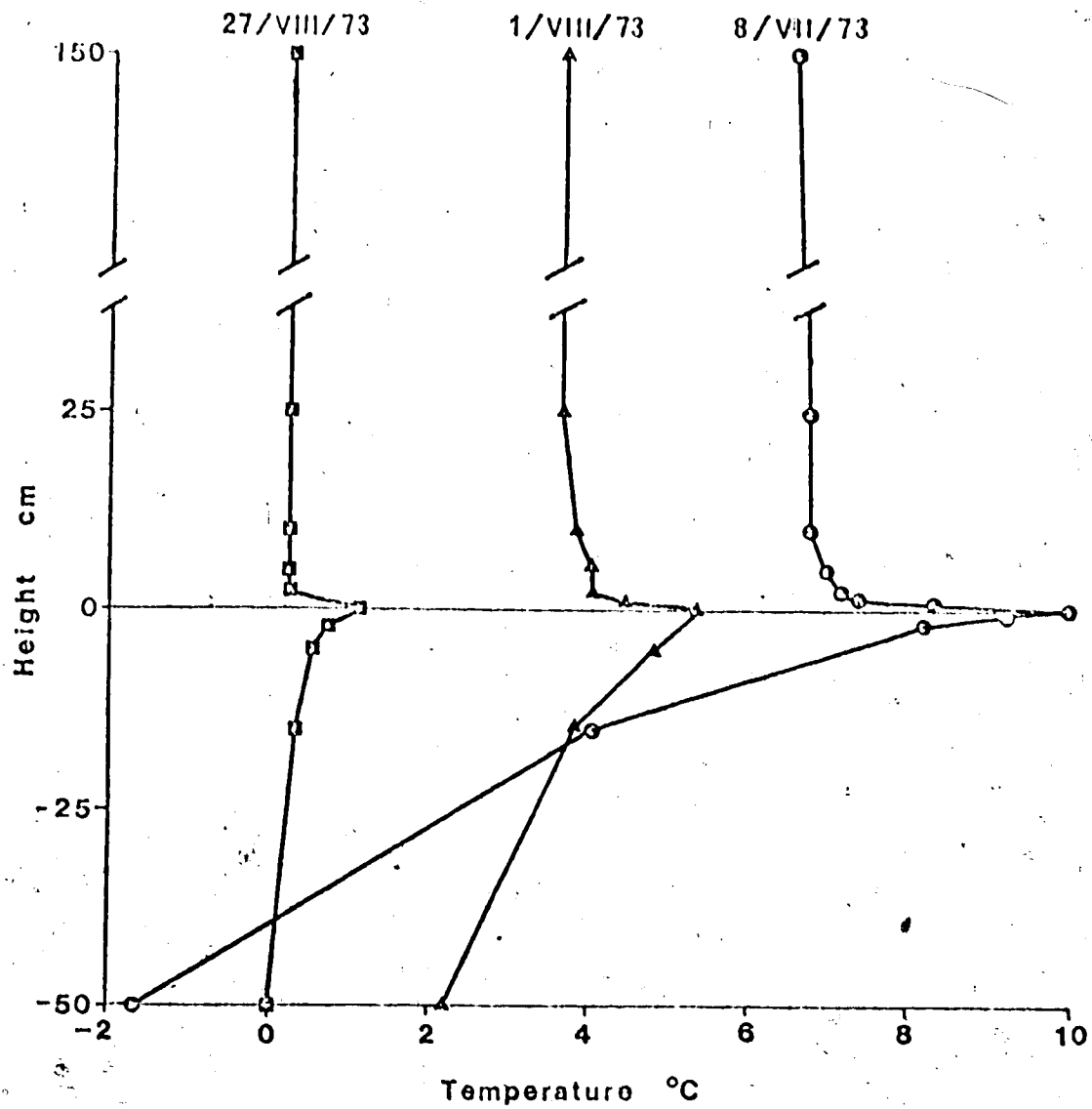
Figure 7. Temperature profiles at the Lichen-Moss-Ruch community for selected periods in 1973. Values are 5 day means.
