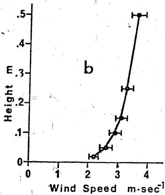
Figure 10. Wind profiles during periods of moderate wind speed ( 3-5 \text{ m sec}^{-1} @ .50 \text{ cm} ) at the Lichen-Moss-Rush (a) and Moss-Lichen-Rush (b) communities. Values are means \pm 95% confidence limits.
