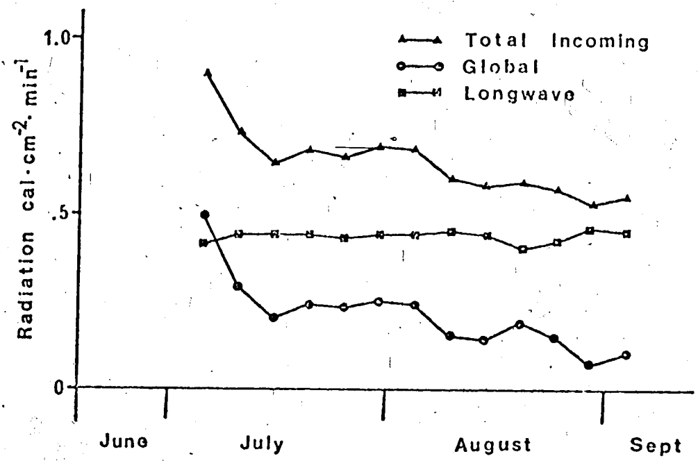
Figure 3. Total incoming radiation and its longwave and shortwave components during 1973. Values are weekly means.
