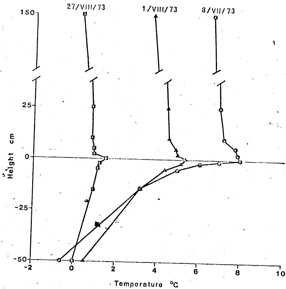
Figure 8. Temperature profiles at the Moss-Lichen-Rush community for selected periods in 1973. Values are 5 day means.
