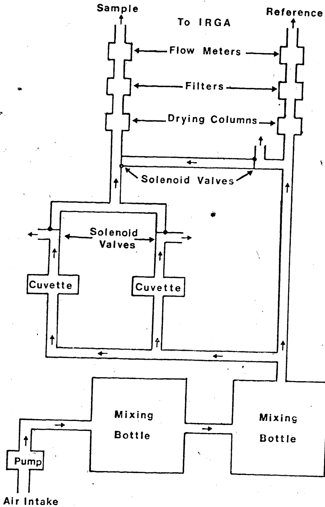
Figure 23. Open gas flow system used in both the field and laboratory.
