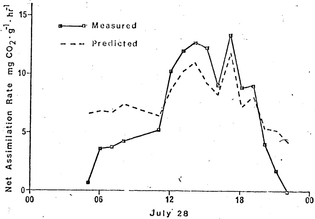
Figure 31. Comparison of net assimilation rate predicted using the laboratory model and field conditions and that measured under field conditions.
