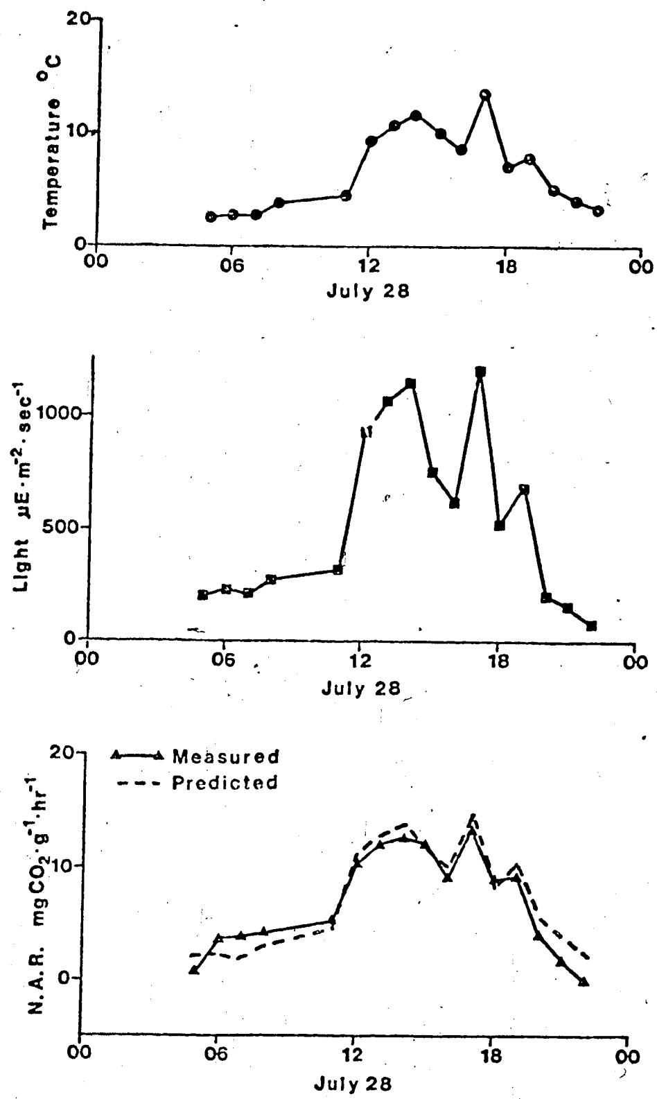
Figure 25. Net assimilation rate of Luzula confusa and environmental conditions during July 28, 1975.
