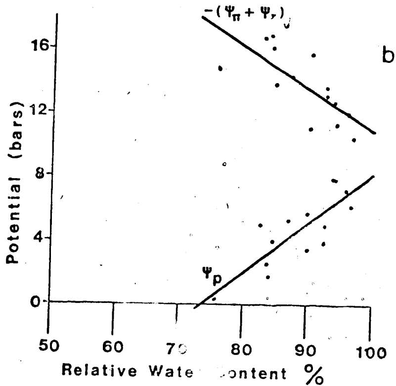
Figure 22. Osmotic plus matric potential ( \Psi_{\pi} + \Psi_r ) and turgor potential ( \Psi_p ) versus relative water content at the beginning (a) and end (b) of a laboratory growing period.
