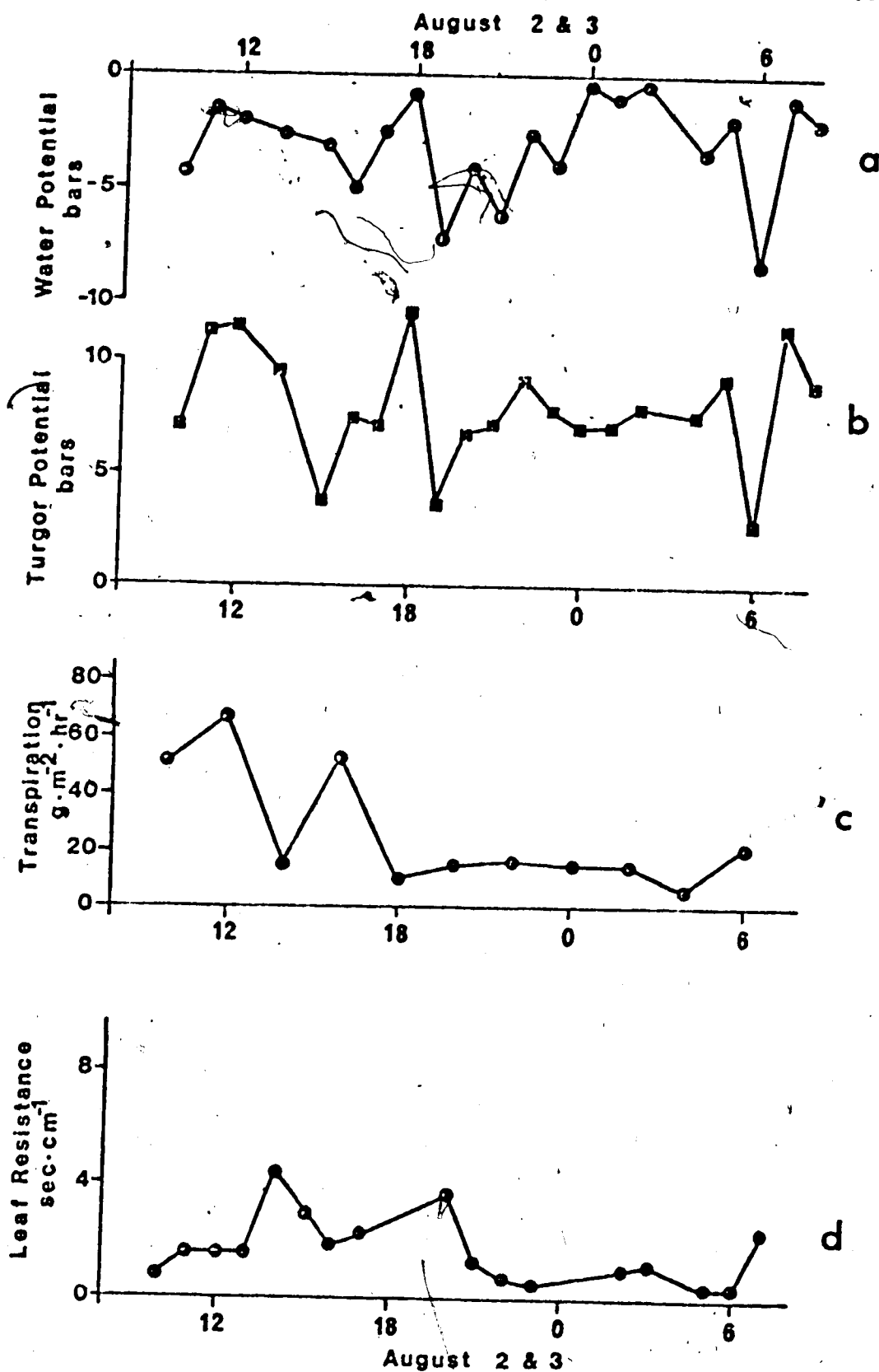
Figure 21. Leaf water potential (a), turgor potential (b), transpiration (leaf area basis) (c), and leaf resistance to water flux (d) of Luzula confusa during August 2 and 3, 1974.
