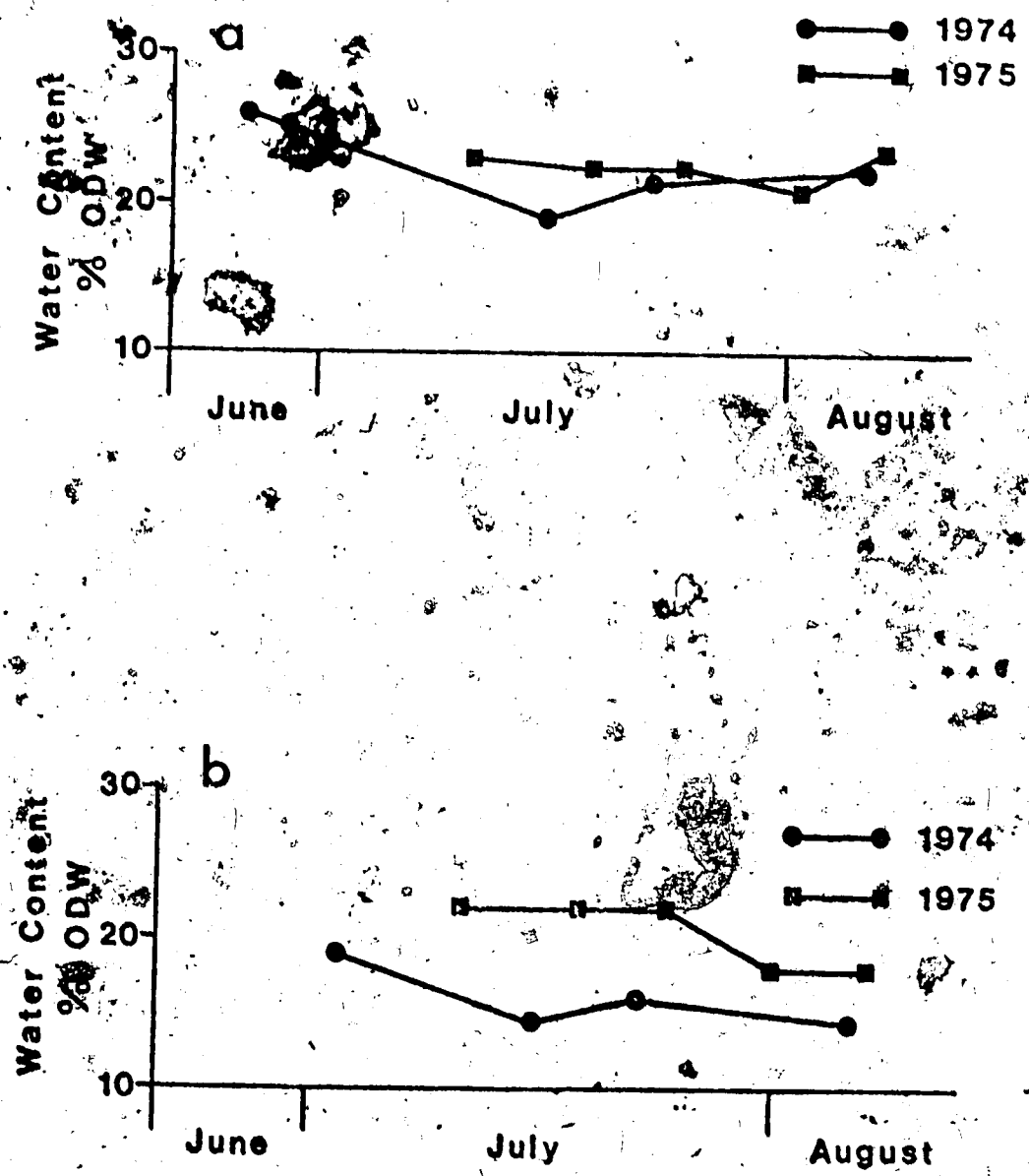
Figure 14. Soil moisture (0-5 cm) of the Moss-Lichen-Rush (a) and Lichen-Moss-Rush (b) communities during the summers of 1974 and 1975. Values are averages of 4 measurements.
