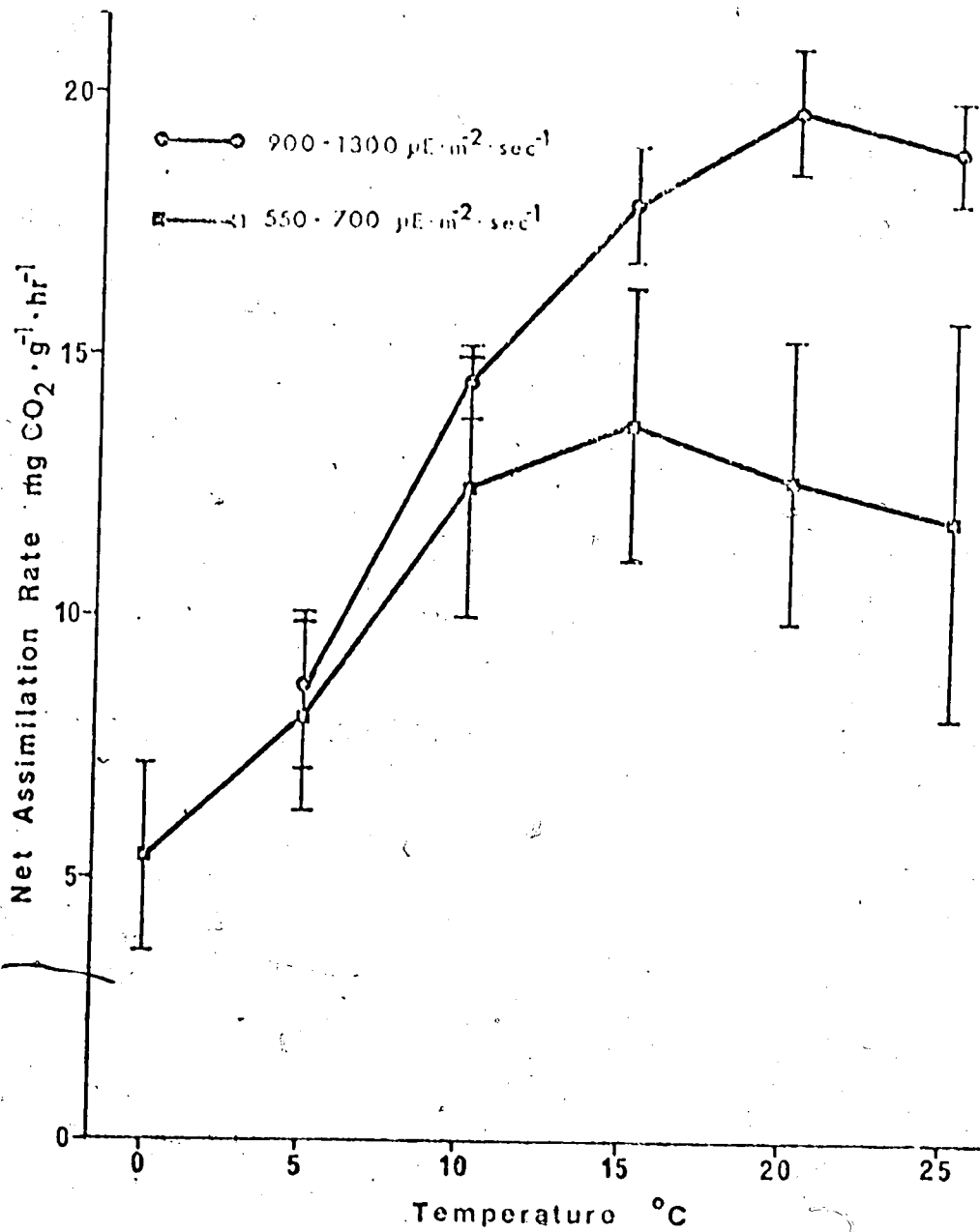
Figure 27. Net assimilation rate of Luzula confusa versus temperature at two different light levels. All points are means with 95% confidence limits.
