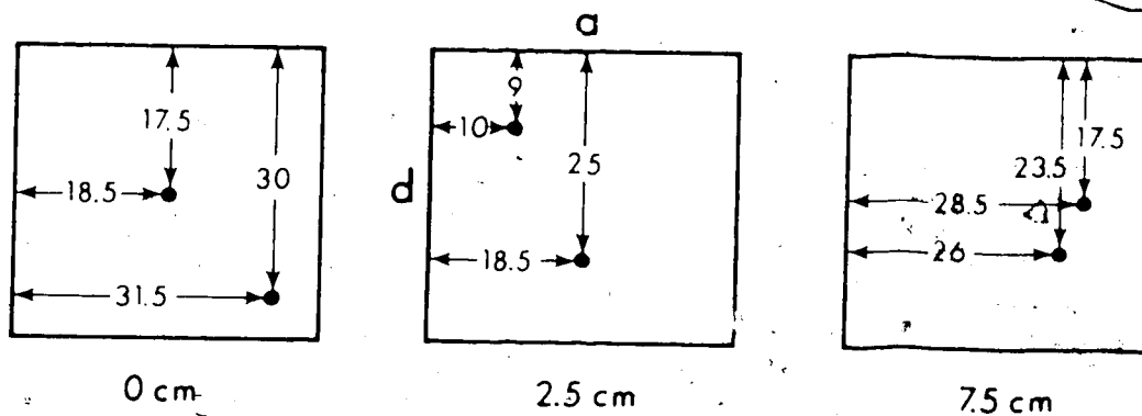
FIGURE 4.3 Load positions at each of the three levels chosen in the domestic microwave oven. a = 37 cm and d = 35 cm.
