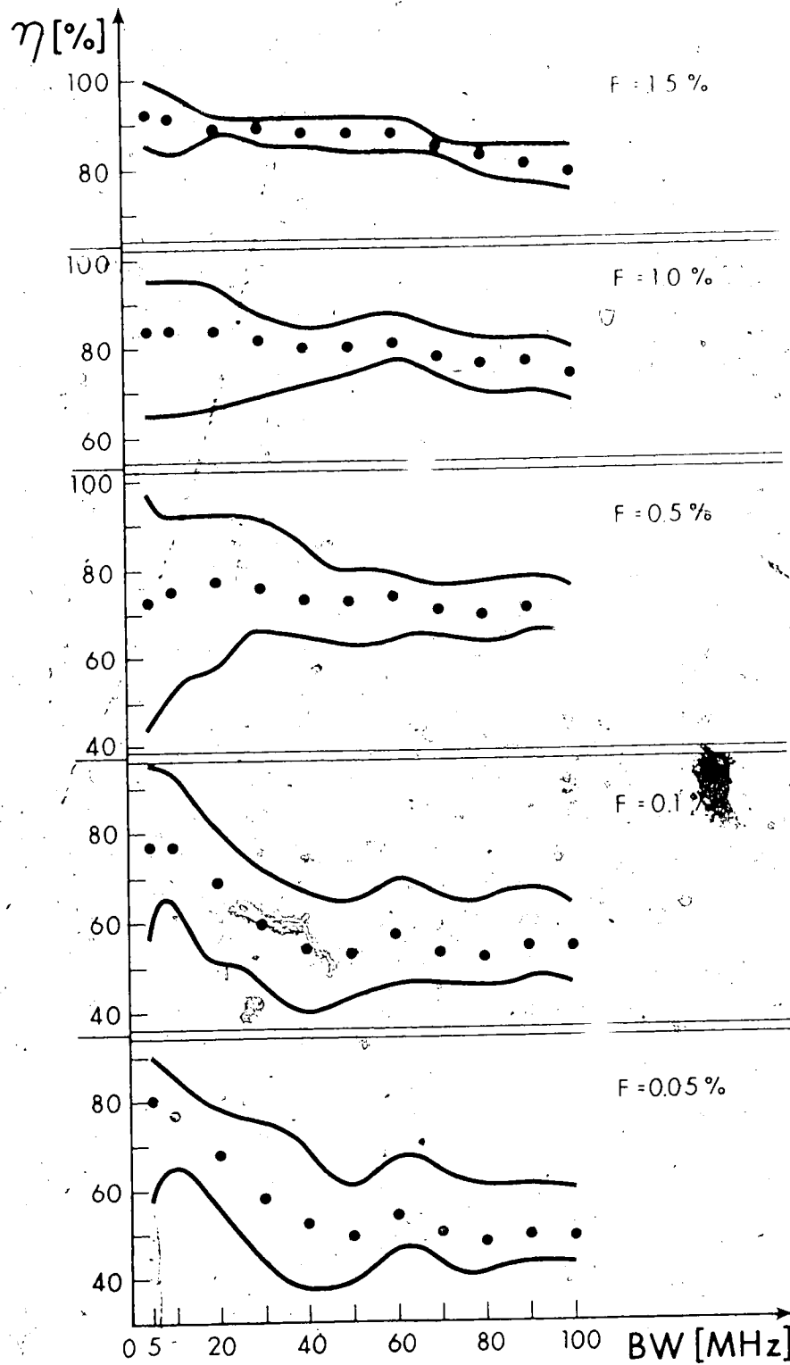
FIGURE 4.8 Relative circuit efficiencies for the experimental cavity, for different source bandwidths swept at constant input power.
