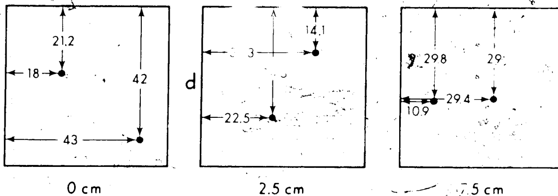
FIGURE 4.1 Load positions at each of the three levels chosen in the experimental cavity. a = 52 cm and d = 50 cm.
