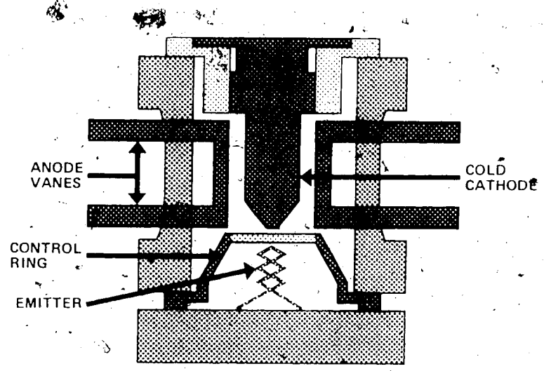
FIGURE 5.1 Cross section of a voltage tunable magnetron.
