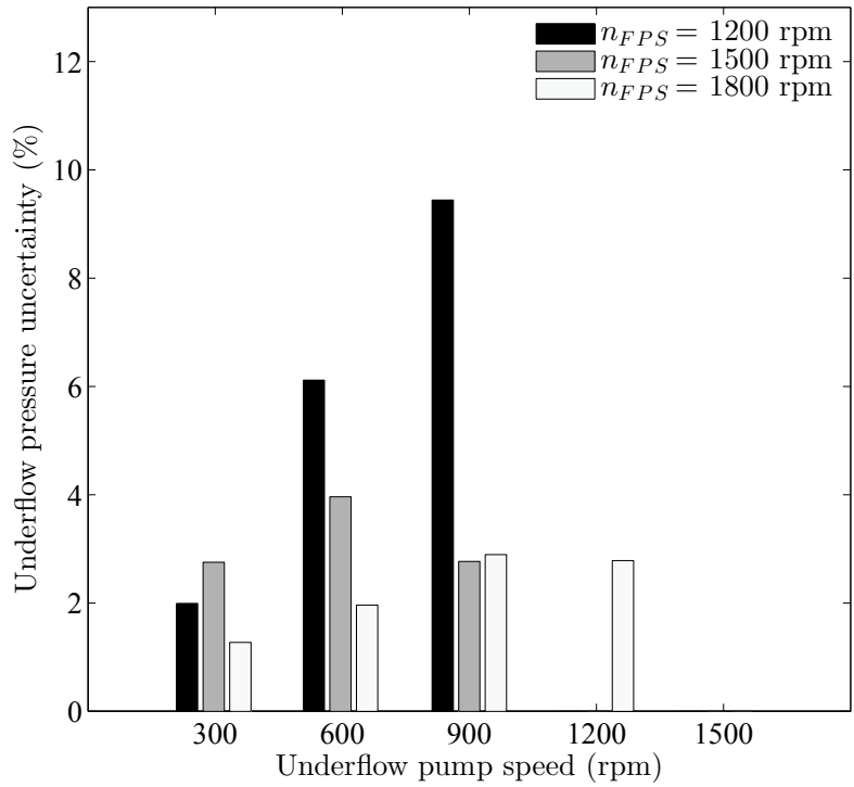
Figure 3.16: Effect of underflow pumping on the total uncertainty of the measured underflow pressure; c = 0.1\%v/v .
