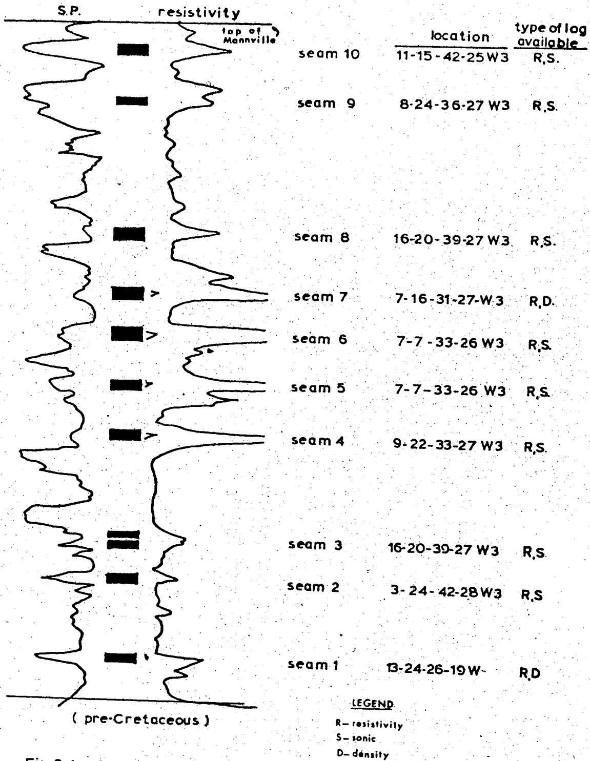
Fig 3.4 COMPOSITE LOG SHOWING RELATIVE POSITION OF SEAMS.
