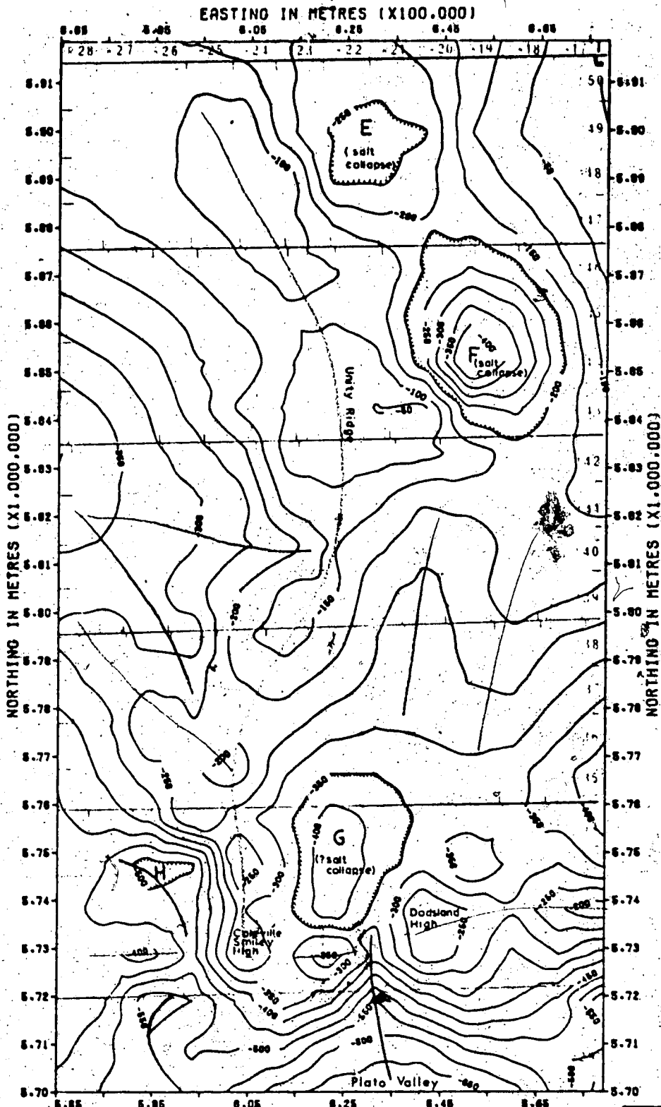
STRUCTURAL MAP OF THE BASE OF MANNVILLE.
