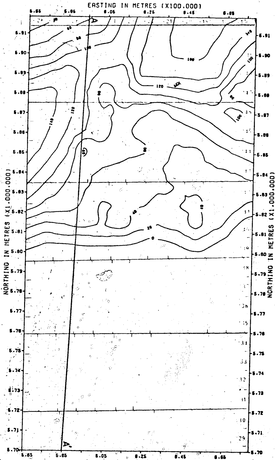
ISOPACH MAP OF THE DINA MEMBER.
