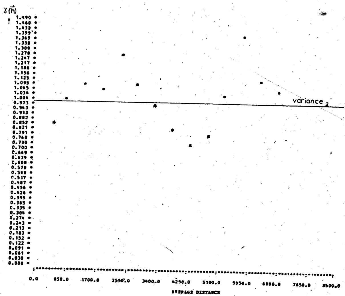
Fig 8.8 VARIOGRAM with direction = 90° - 270°
