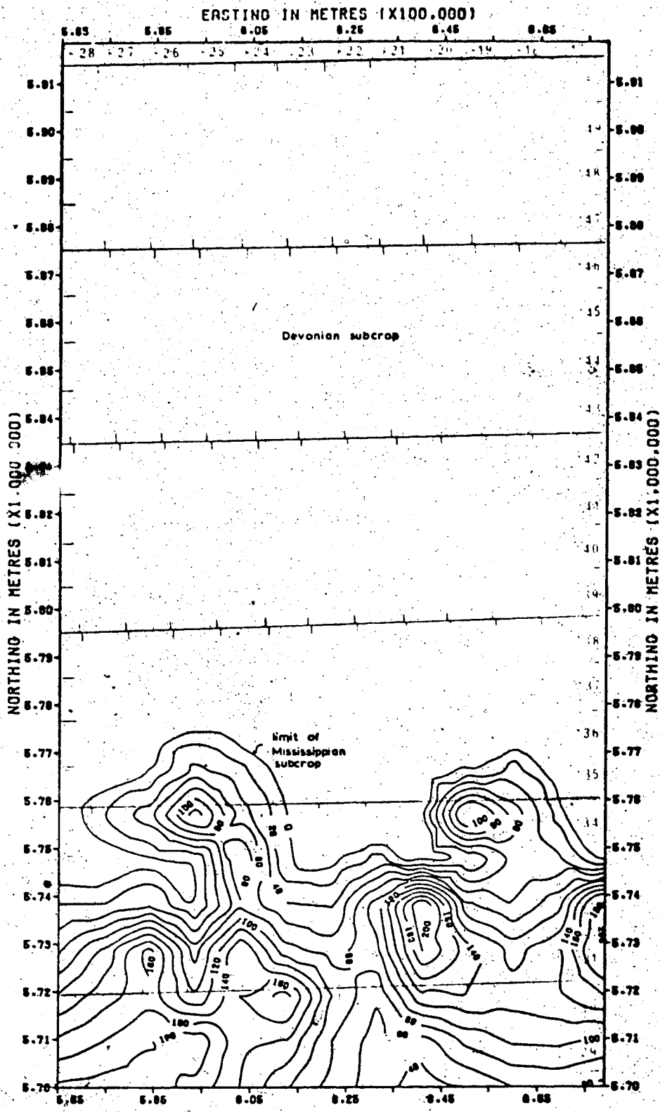
ISOPACH MAP OF MISSISSIPPIAN.
