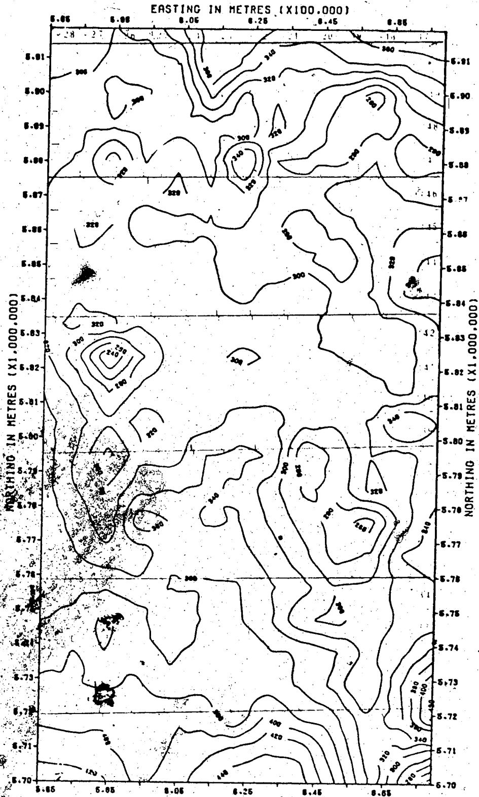
ISOPACH MAP: BASE OF FISH SCALES TO TOP OF MANNVILLE.
