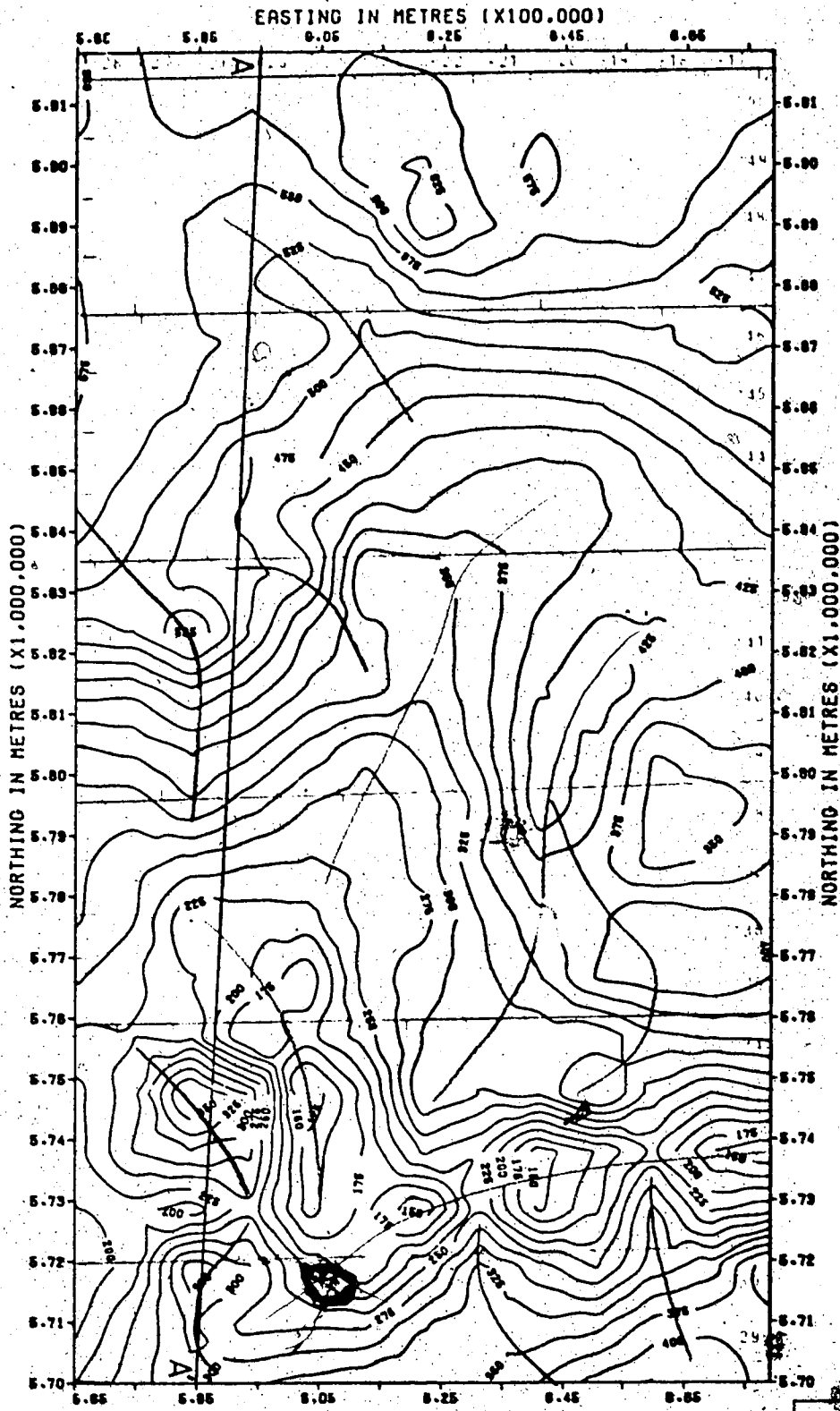
ISOPACH MAP OF THE MANNVILLE GROUP.
