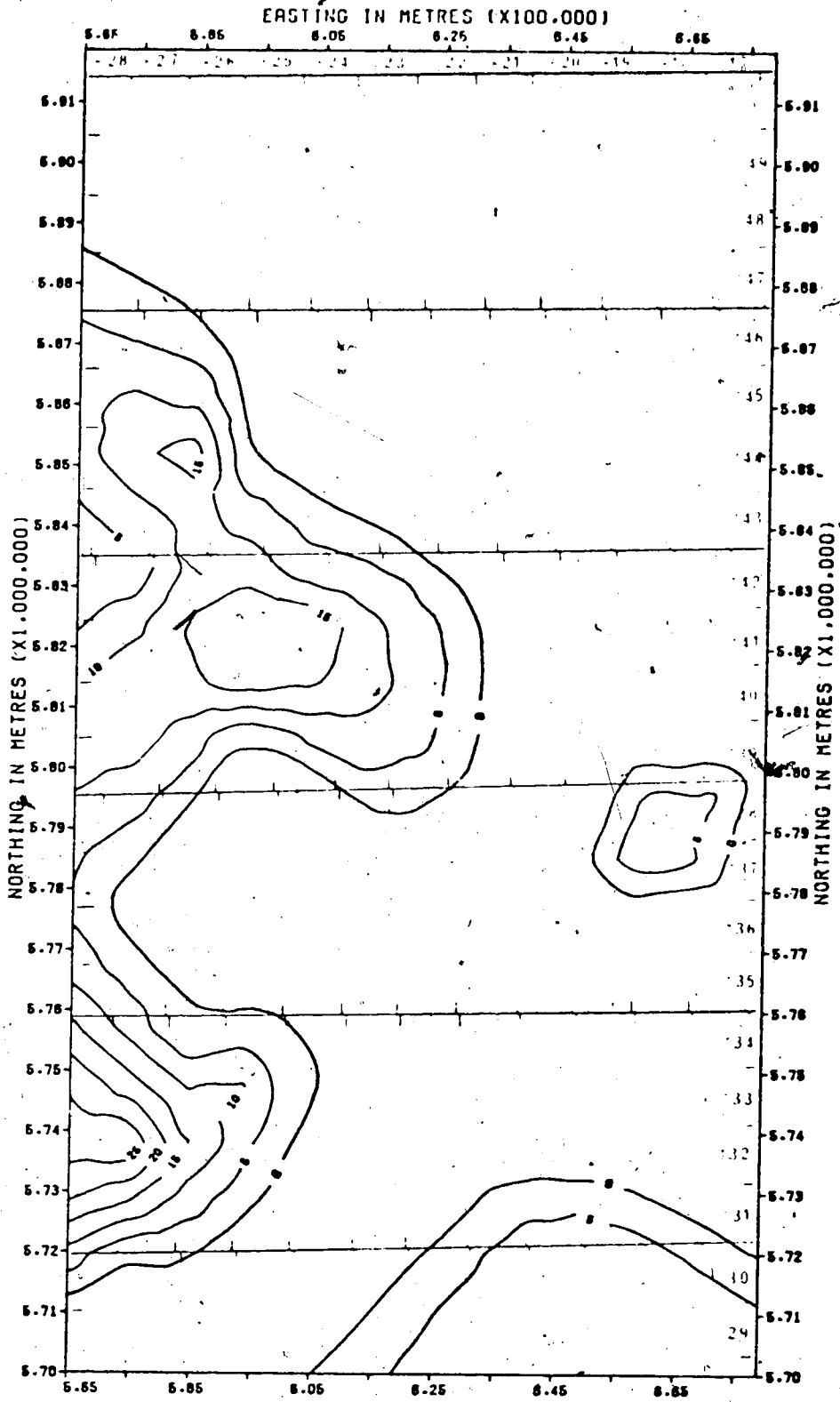
RELATIVE STANDARD DEVIATION OF COAL SEAMS.
