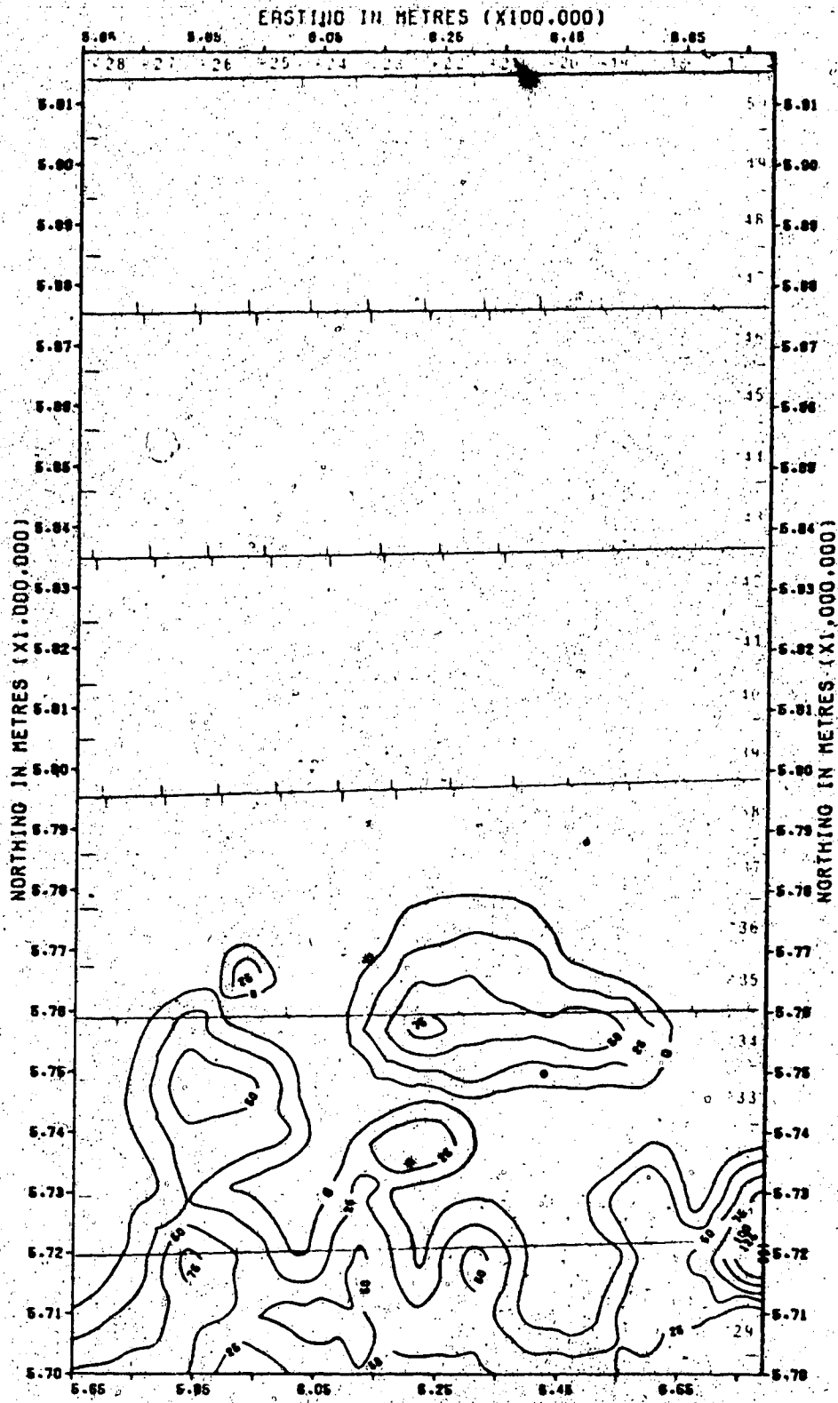
ISDPACH MAP OF THE DEVILLE MEMBER.
