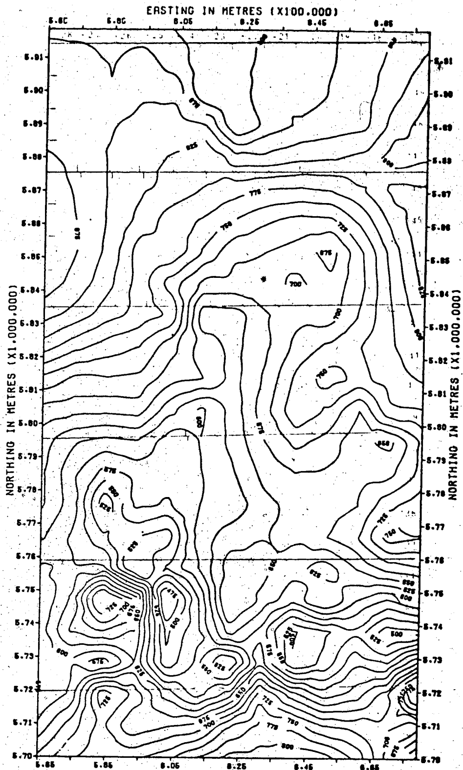
ISOPACH MAP: BASE OF FISH SCALES TO BASE OF MANNVILLE.
