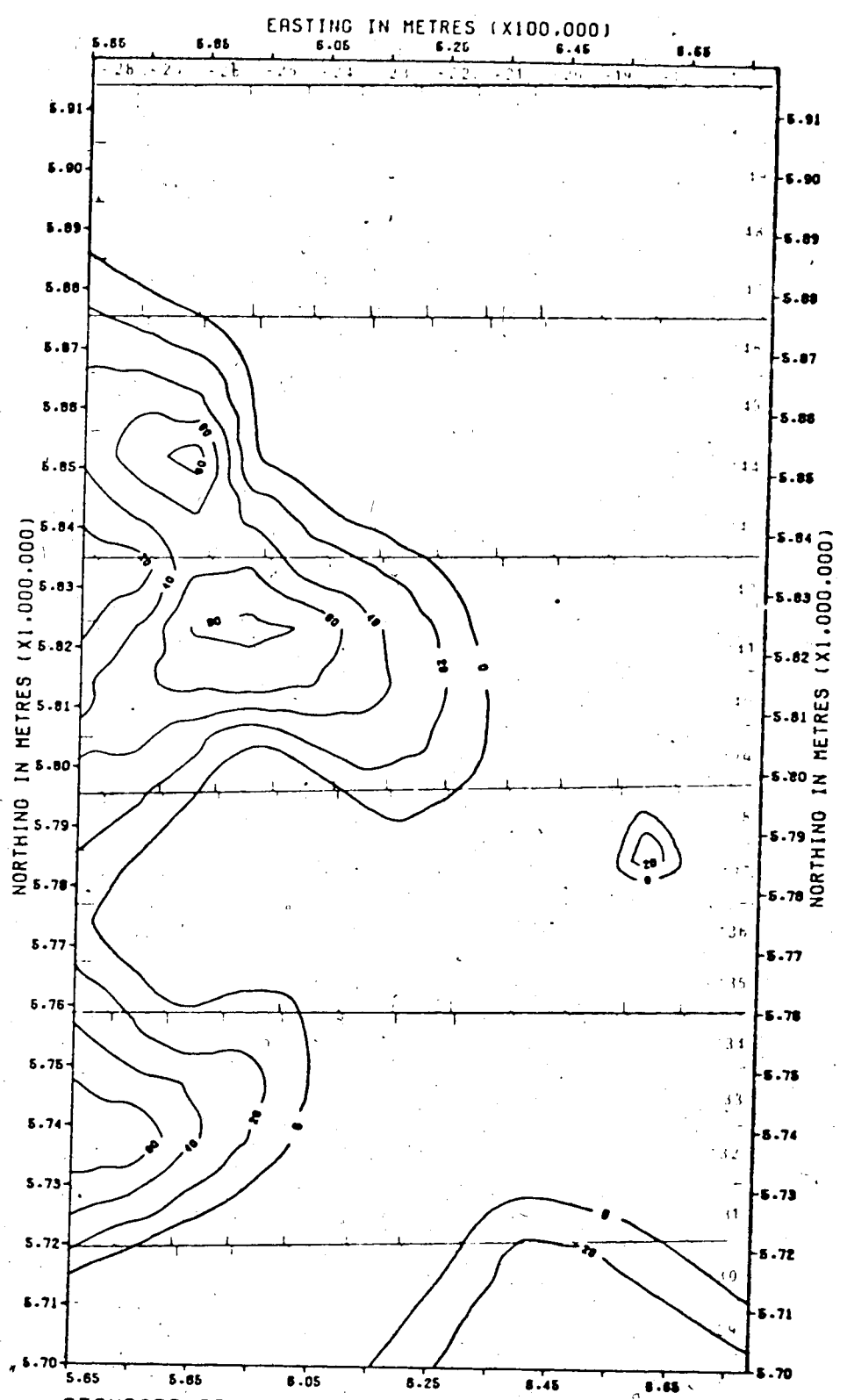
STANDARD DEVIATION MAP OF COAL SEAMS.
