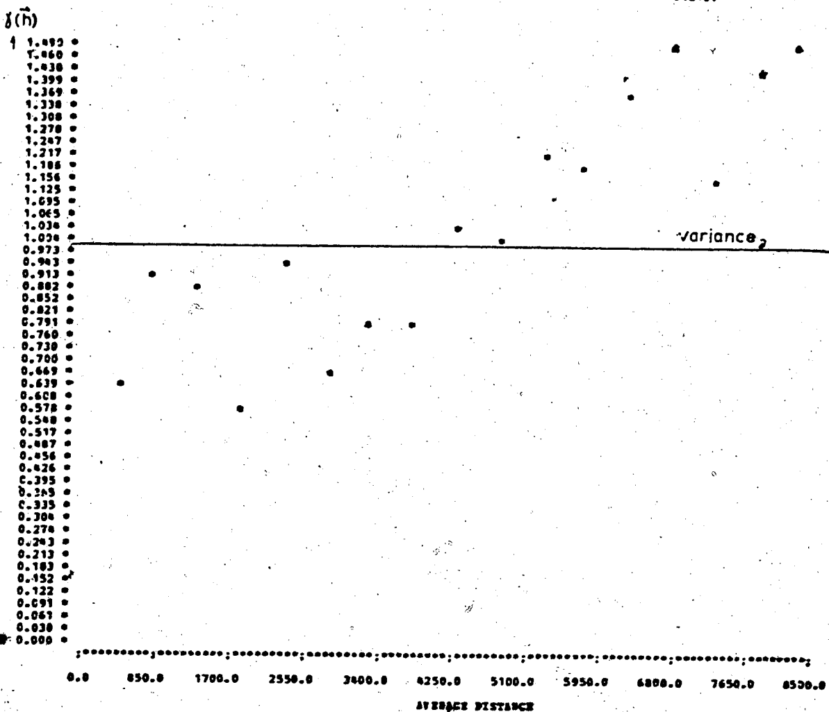
Fig 8.10 VARIOGRAM with direction = 150° ~ 330°
