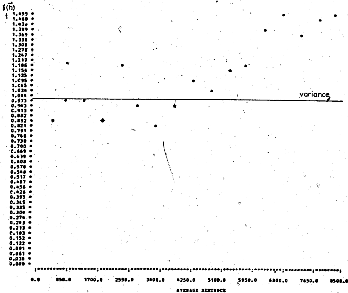
Fig 8.9 VARIOGRAM with direction = 120° or 300°
