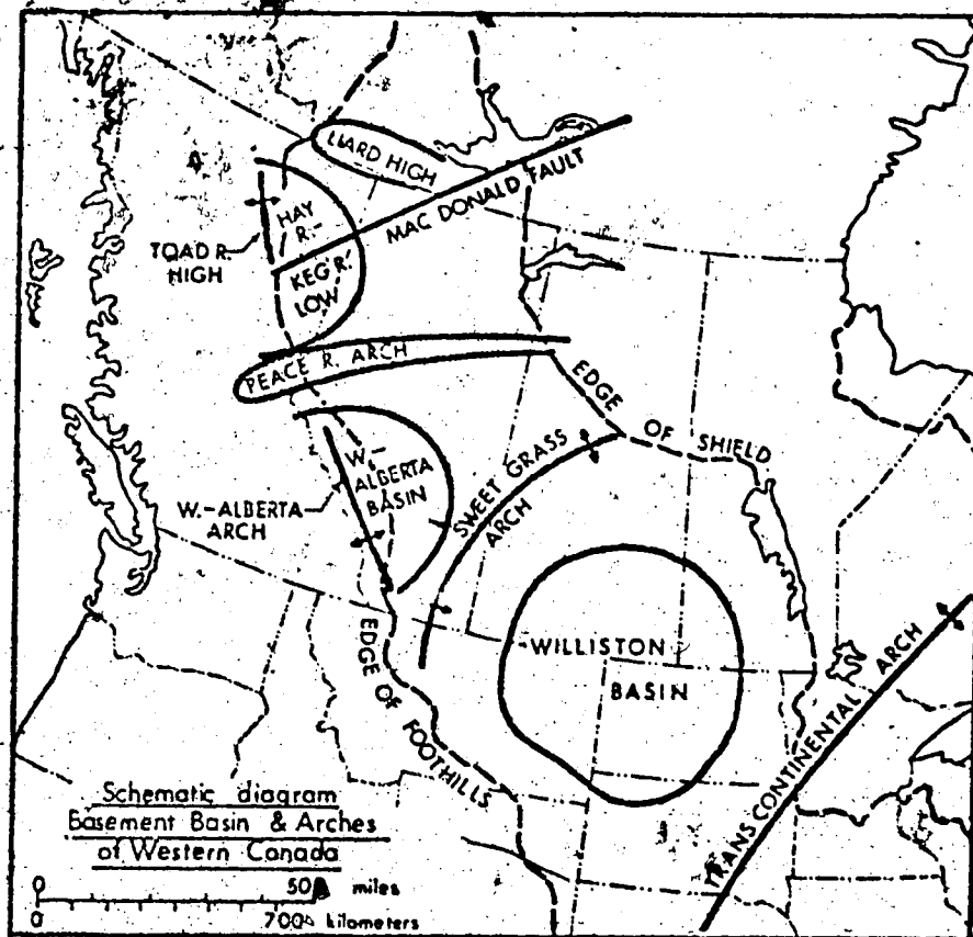
Fig 5.6 SCHEMATIC DIAGRAM of PRECAMBRIAN BASMENT FEATURES of WESTERN CANADA. (After Stelck, 1975)
