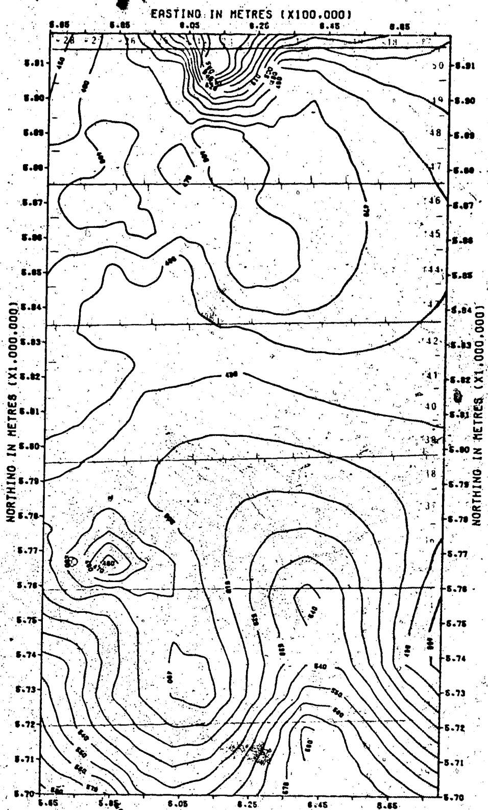
ISOPACH MAP: BASE OF FISH SCALES TO SEAM 8.
