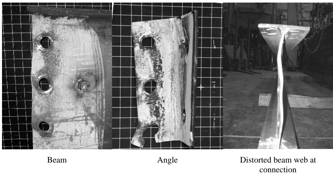
Figure A-24 Test specimen 1L9a
