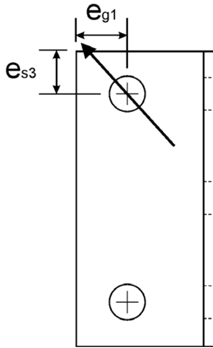
b) Bolt Force Crosses the Top End
