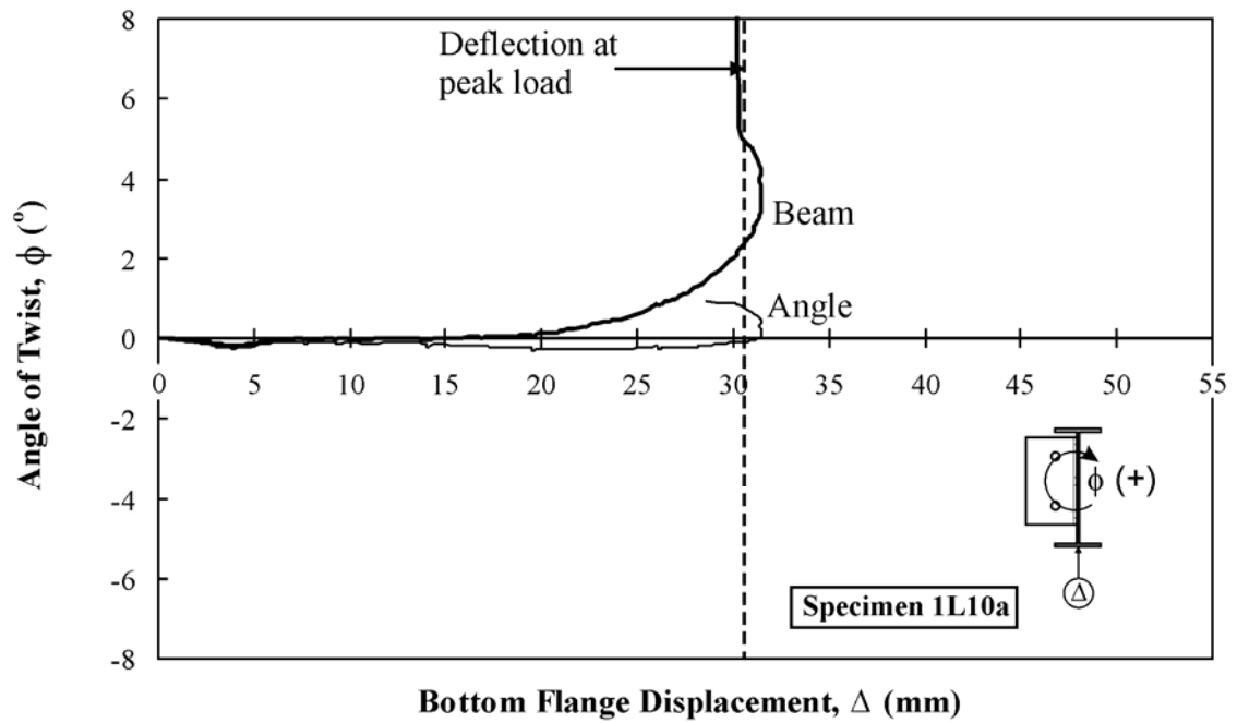
Figure B-54 Twist vs. Bottom Flange Displacement, Test Specimen 1L10a
