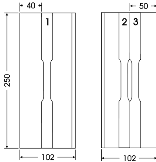
c) Location of Coupons on Angle L102x102x6.4
