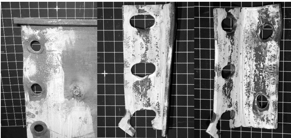
Beam
