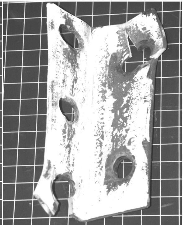
b) Test Specimen 1L2
