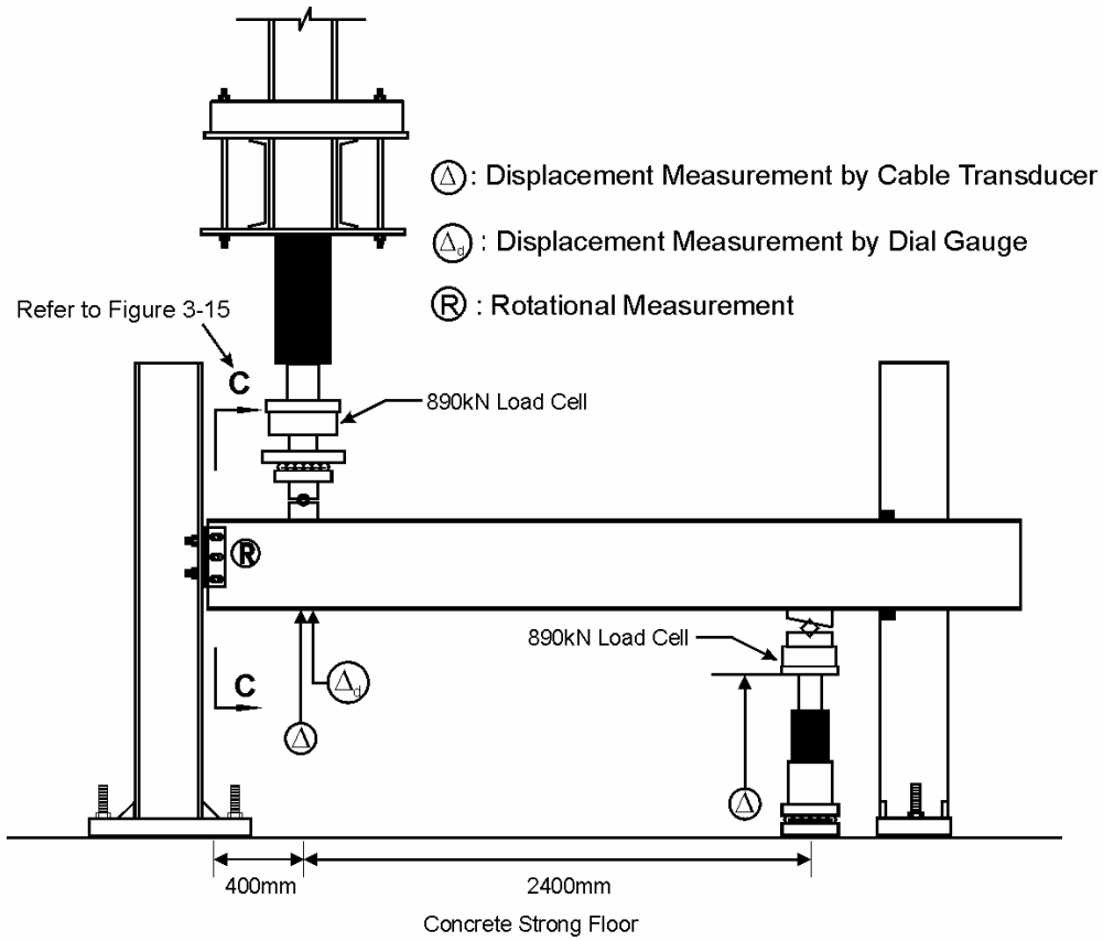
Figure 3-14 Instrumentation
