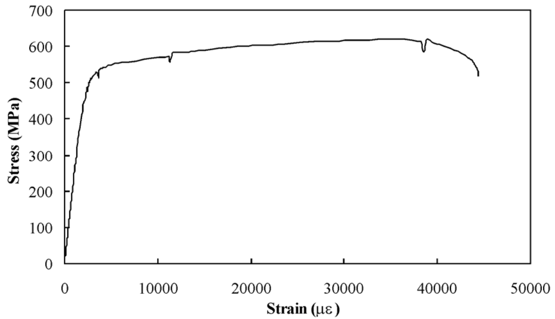
b) Tested Angles (Coupon V1)
