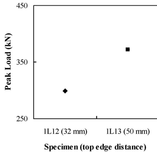
Figure 4-35 Effect of Edge Distance on Capacity of Connection that Failed in the Leg Connected to the Column
