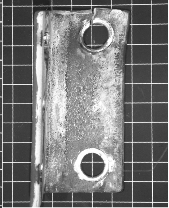
b) Test Specimen 1L7
