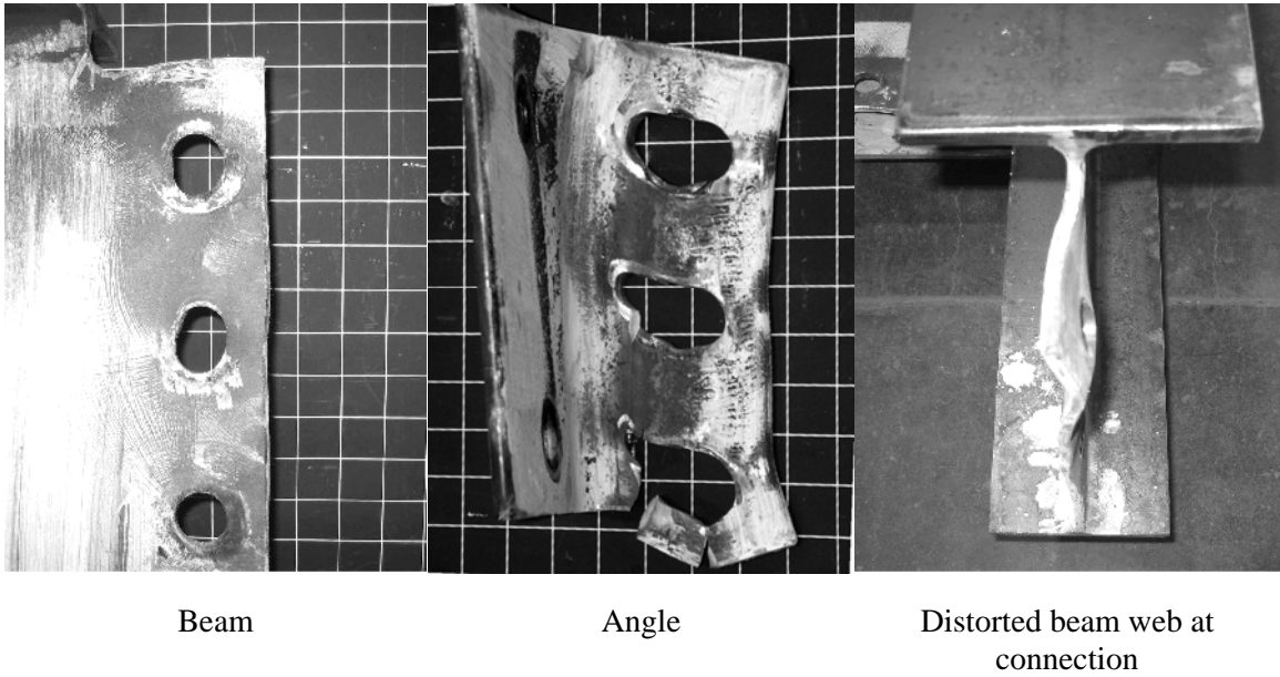
Figure A-23 Test specimen 1L8a
