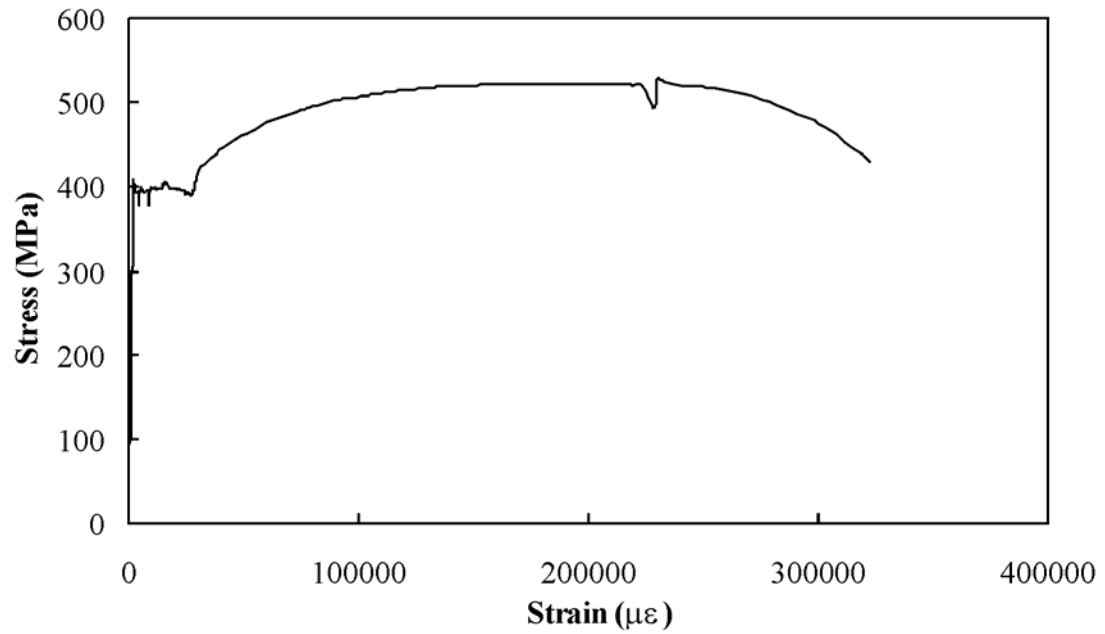
a) Beam Material (Coupon A1)
