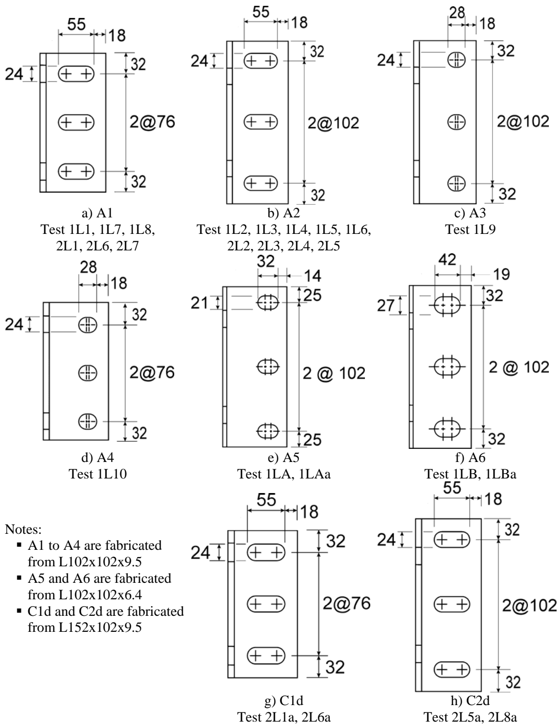
Figure 3-2 Nominal Angle Dimensions
