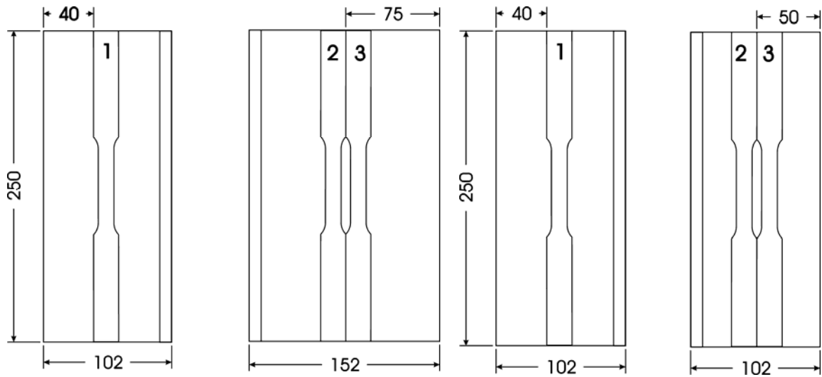
a) Location of Coupons on Angle L152x102x9.5
