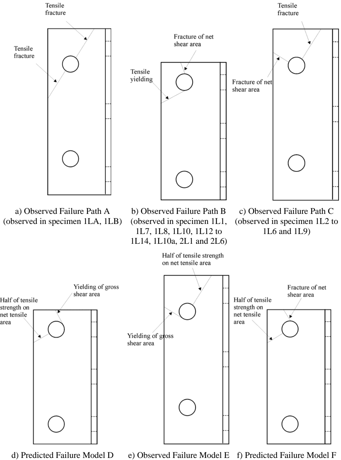
Figure 5-4 Observed Failure Paths and Predicted Failure Model
