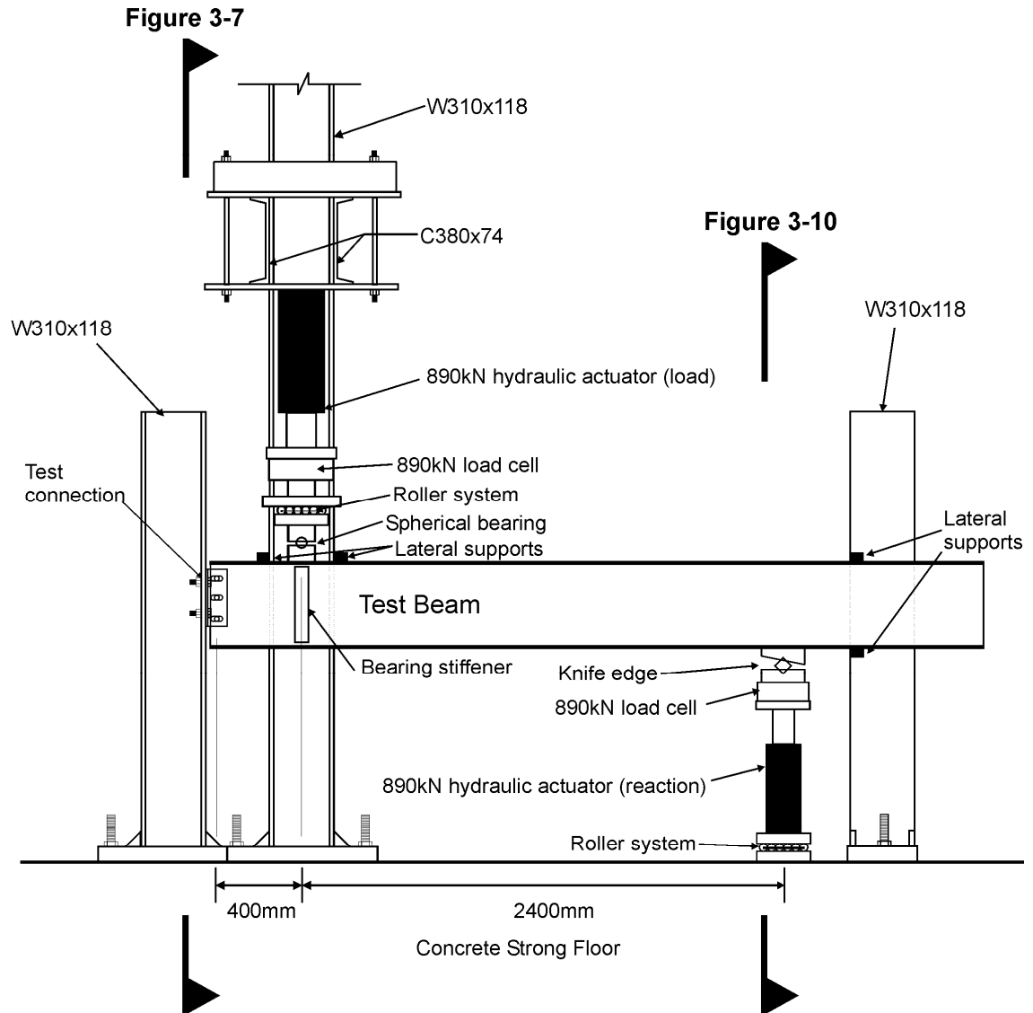
Figure 3-4 Elevation View of Test Setup
