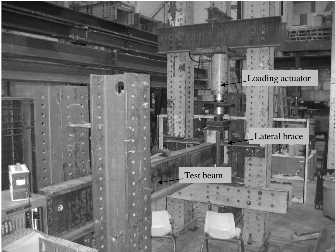
Figure 3-5 Overall Test Setup
