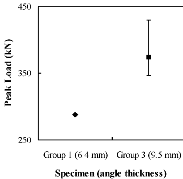
Figure 4-33 Effect of Angle Thickness on Capacity of Connection that Failed in the Leg Connected to the Column
