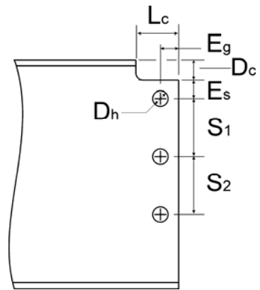
d) Typical Beam with Coped Flange
