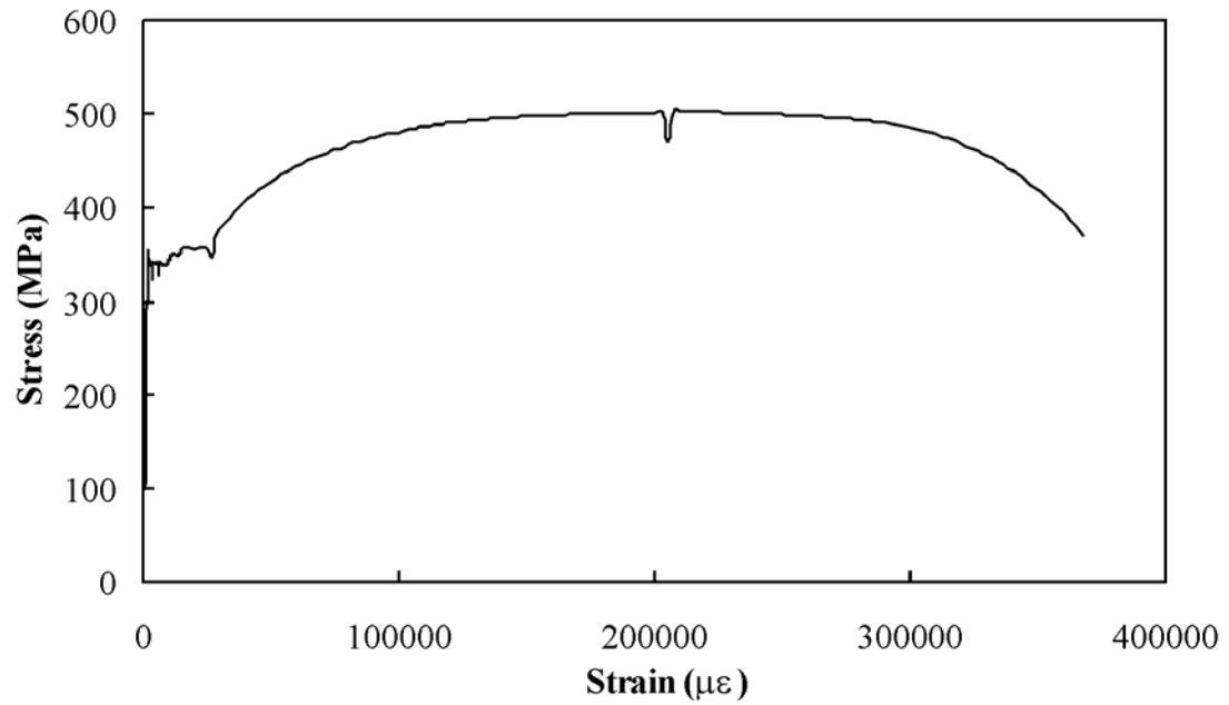
c) Virgin Angles (Coupon Y1)
