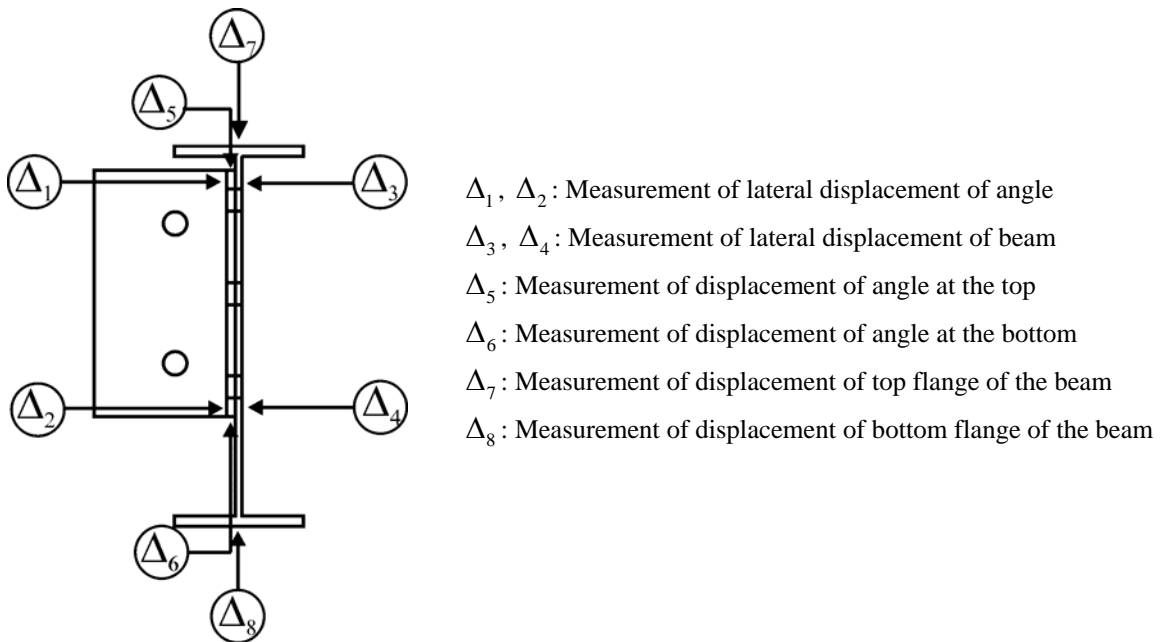
Section C-C in Figure 3-14
