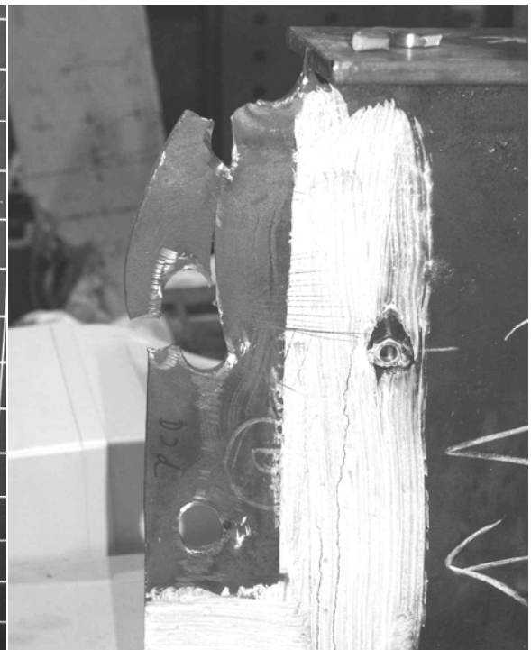
b) Test Specimen 2L8a
