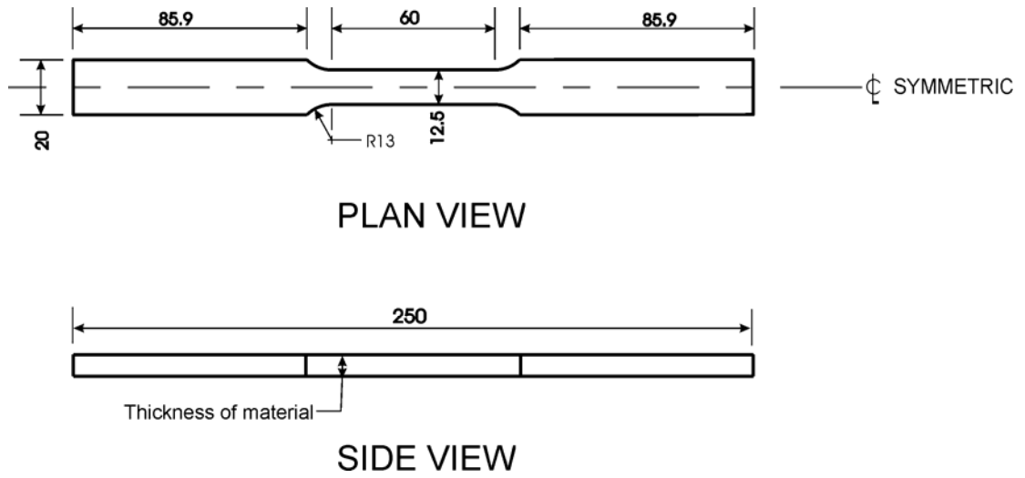
Figure 3-16 Typical Tension Coupon Dimensions
