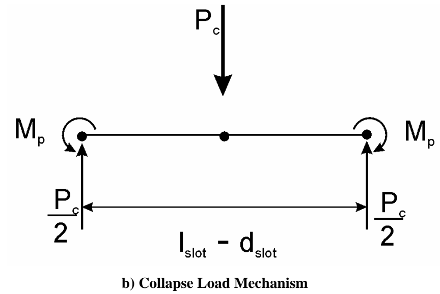
Figure 5-1 Collapse Load Capacity of End Distance in a Slotted Hole Connection
