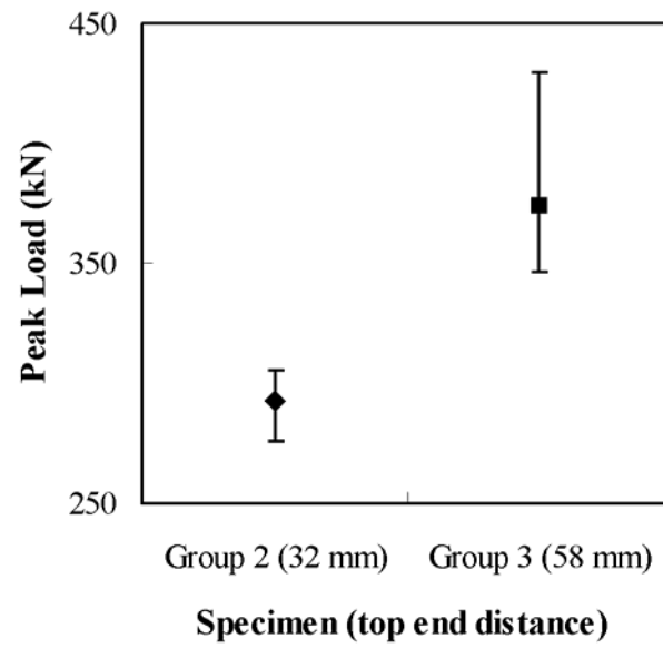
Figure 4-34 Effect of Top End Distance on Capacity of Connection that Failed in the Leg Connected to the Column
