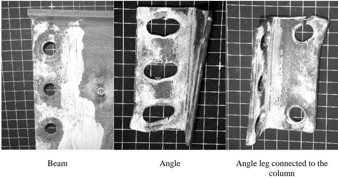
Figure A-5 Test specimen 1L1
