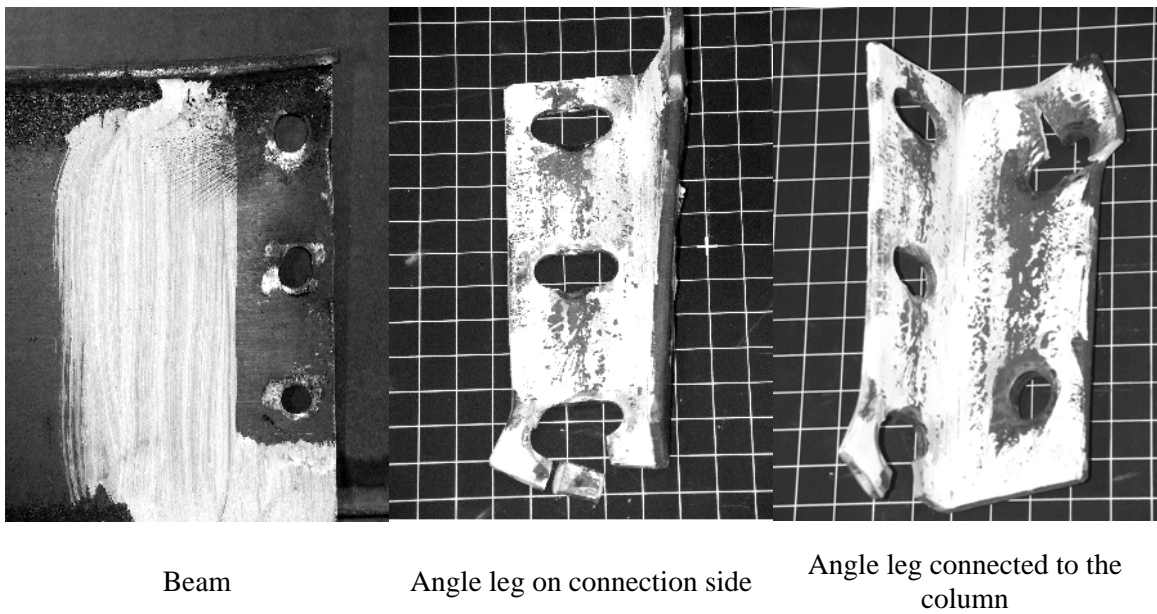
Figure A-6 Test specimen 1L2
