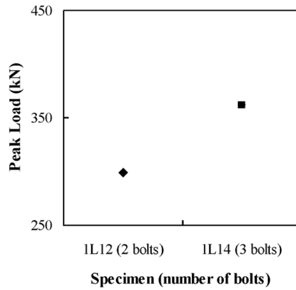
Figure 4-36 Effect of Number of Bolts on Capacity of Connections that Failed in the Leg Connected to the Column
