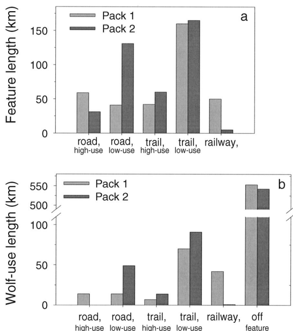
FIG. 3. Length of roads, trails, and railway line (a) within the study area and (b) used by wolves. Seventy-nine percent of the wolf paths were at least 25 m from roads, trails, and the railway line (i.e., off feature).
