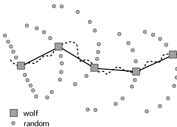
FIG. 1. For the matched case-control logistic regression, 10 controls (random points) were paired with each case (wolf point). Wolf paths (a) were first simplified into a series of wolf points separated by 1000 m (b). To avoid bias potentially associated with the start of each path, we defined the first step as a random point along the first 500 m of the path. To create the controls (c), random turn angles between +90° and -90° were added to the previous direction of travel. Ninety percent of actual wolf turn angles were <90°.
