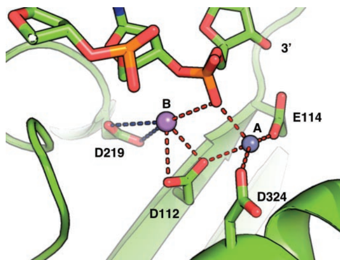
Figure 1. Exonuclease active site of T4 DNA polymerase (21) (PDB: 1NOY). The structure of the exonuclease active site is shown with the four conserved catalytic residues. The two divalent metal ions are shown as spheres. Inter-atomic distances <3.5 Å are shown as red, dashed lines and those >3.5 Å are shown in blue. This figure was made with PyMOL (37).
