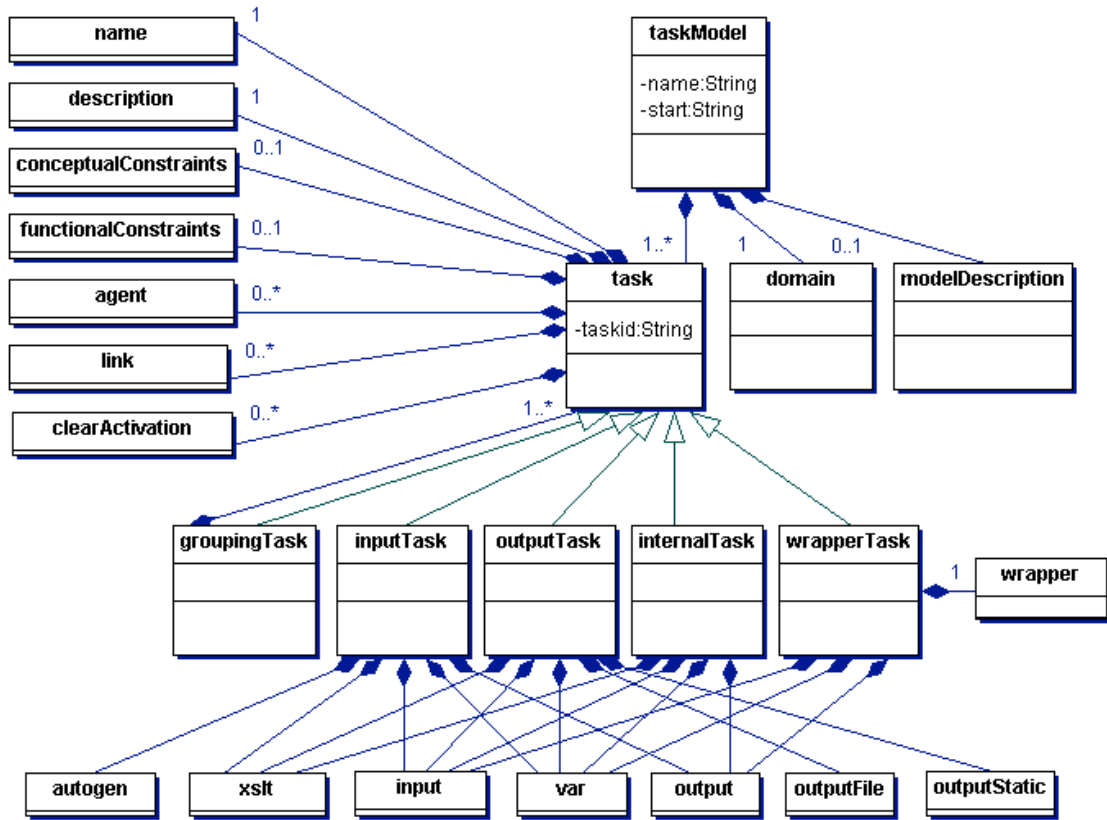
Figure 2: Task Model Schema UML Diagram
