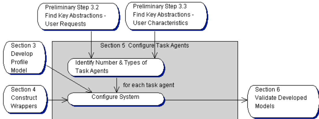
Figure 22: TaMeX Task Agent Configuration Development Activities
