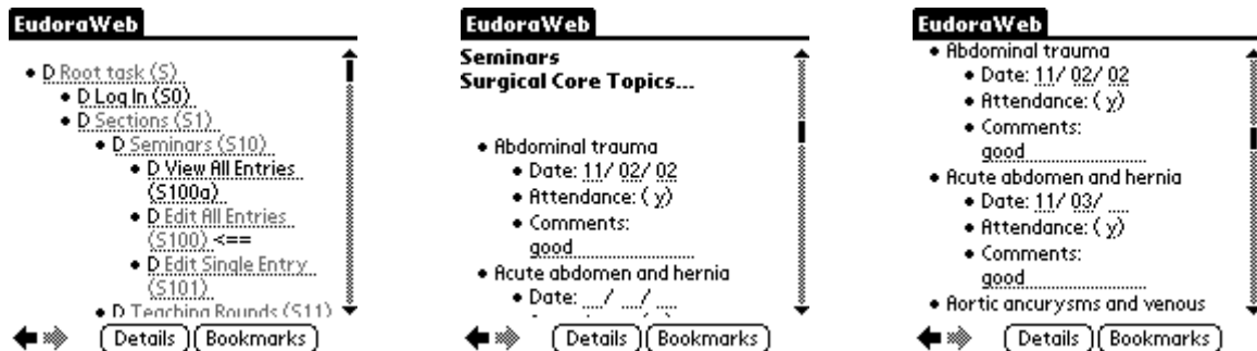
Figure 36: Surgery 446 Mobile Device Version of Edit All Entries (S100)
