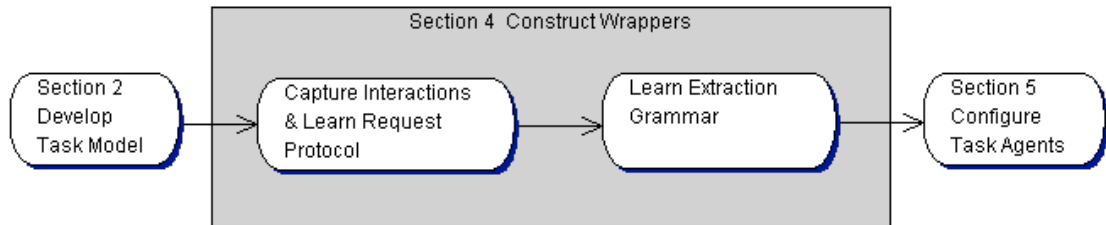
Figure 21: TaMeX Wrapper Construction Activities
