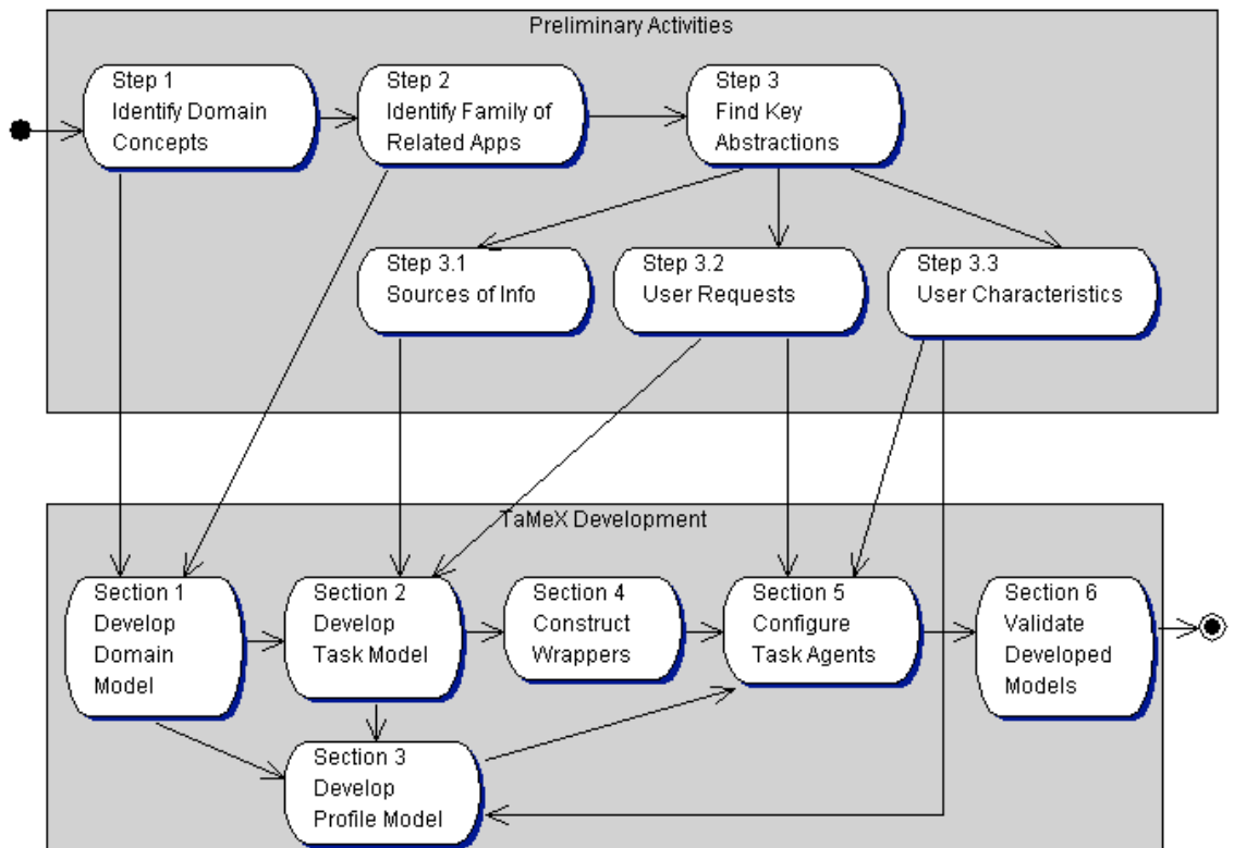
Figure 15: TaMeX Development Activities
