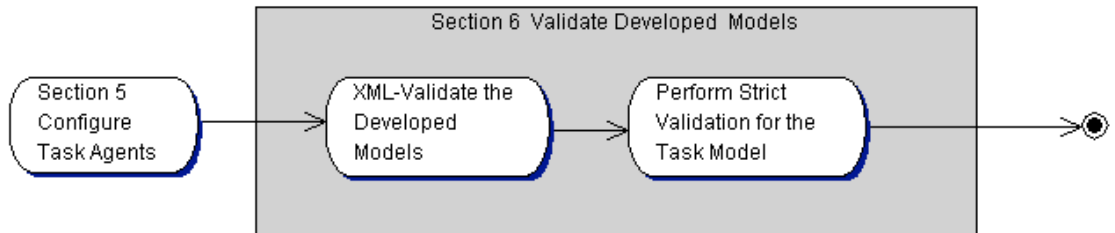
Figure 23: TaMeX Model Validation Development Activities
