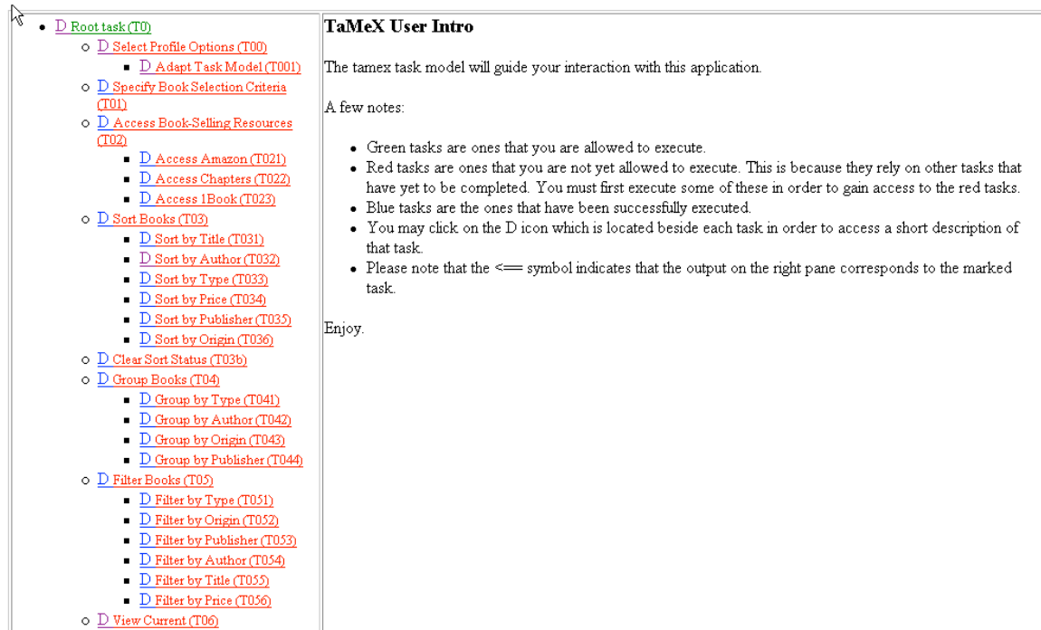
Figure 25: First Task Model Interaction Screen
