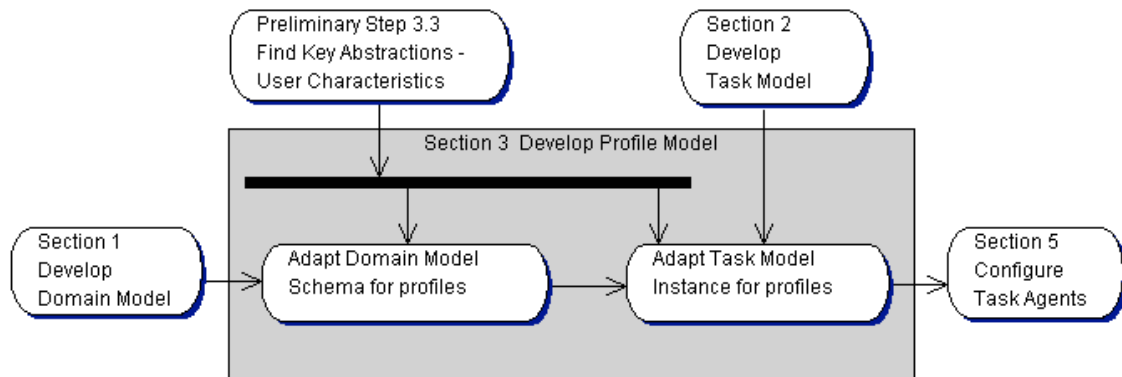
Figure 20: TaMeX Profile Model Development Activities
