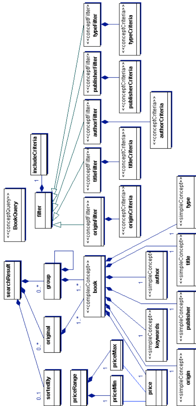
Figure 18: Book-Finding Domain Model Schema UML Diagram
