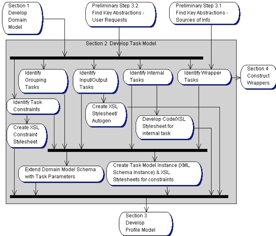
Figure 19: TaMeX Task Model Development Activities
