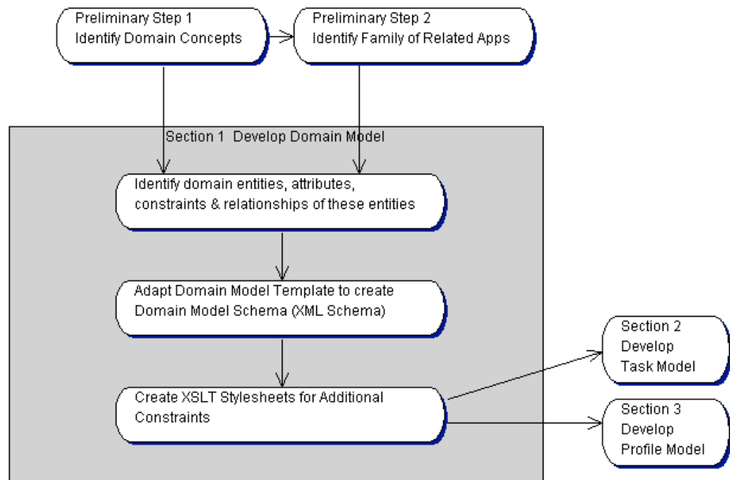
Figure 16: TaMeX Domain Model Development Activities
