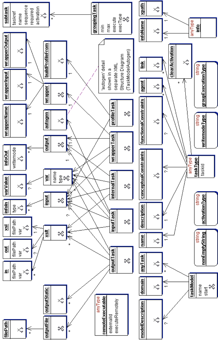
Figure 3: Task Model Schema - XML Structure Diagram
