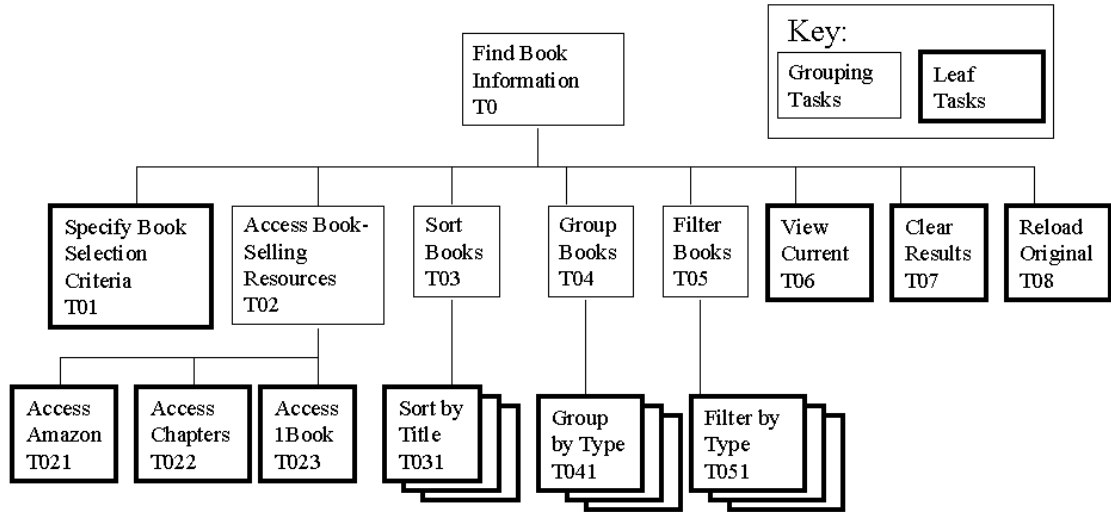
Figure 5: Task Structure for the Book-Finding Application
