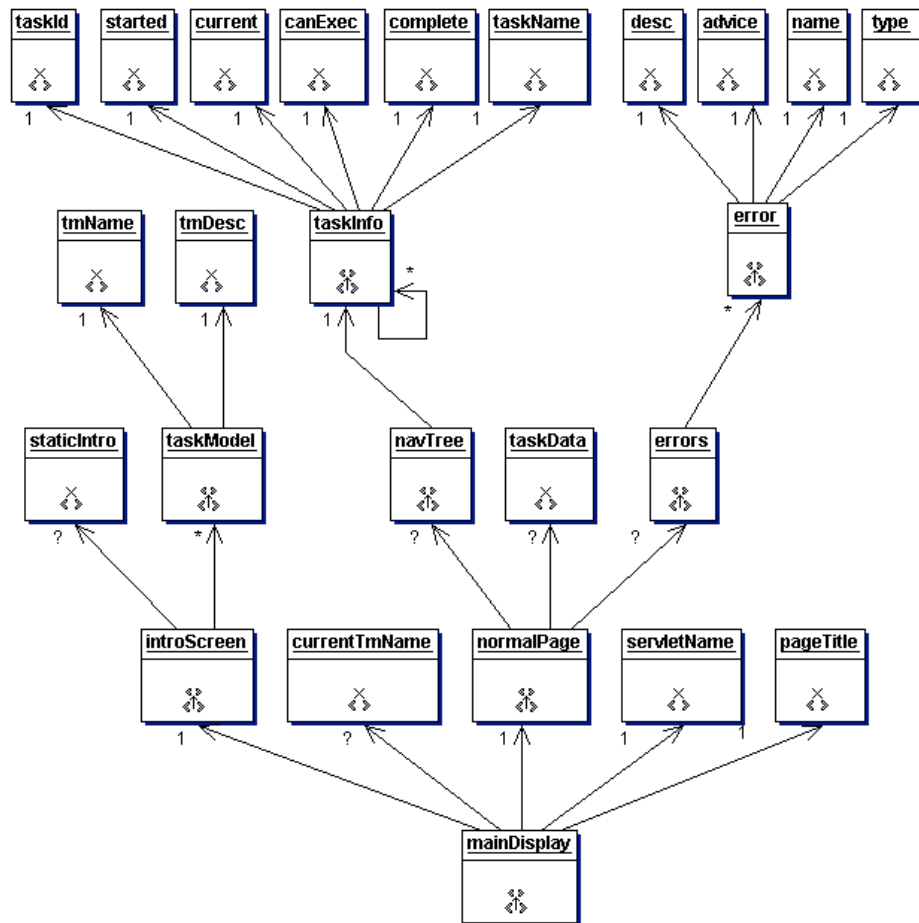
Figure 10: Main Display Schema - XML Structure Diagram
