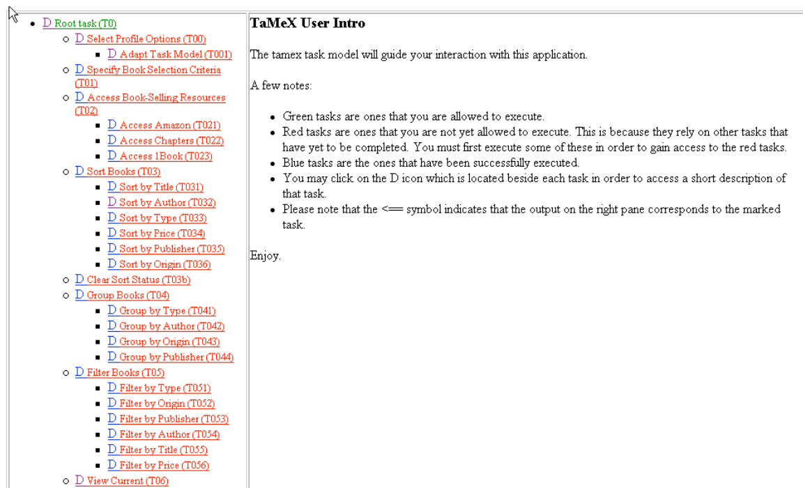
Figure 13: Task Model Interaction Screen
