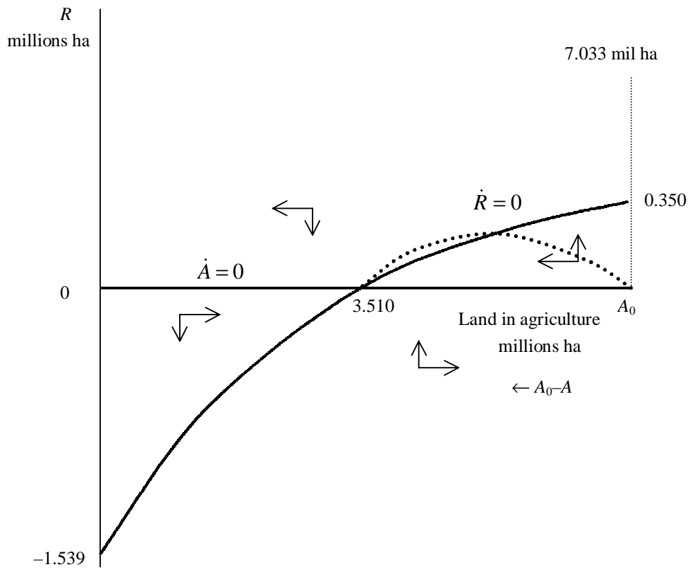
Figure 2: Phase-Plane Diagram of the Optimal Afforestation Path
