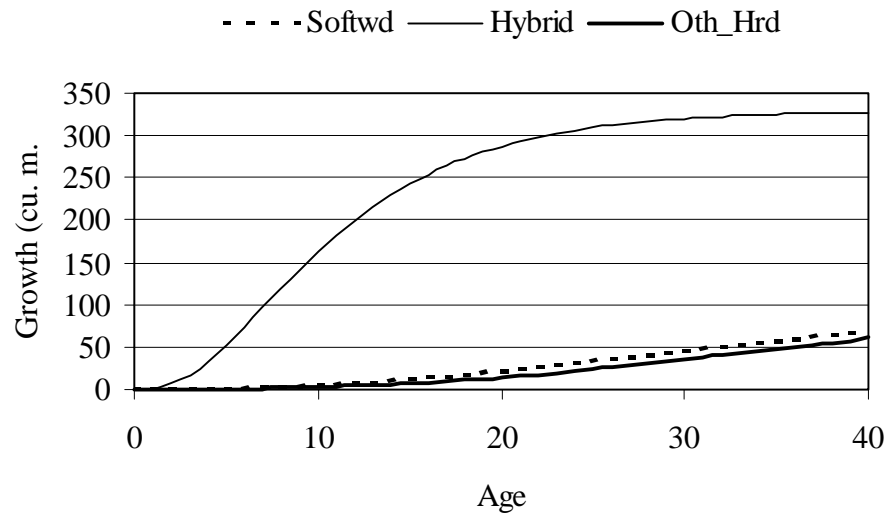
Figure 1: 40-Year Growth for Various Tree Species, Boreal Region, Western Canada
