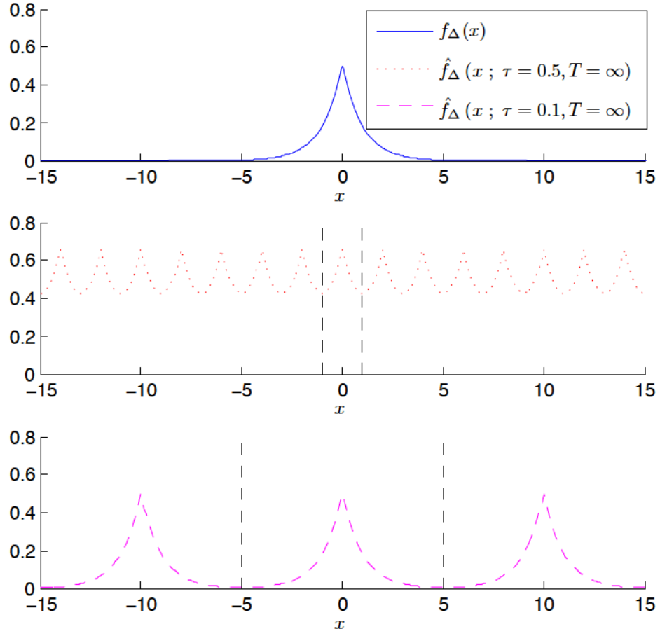
Figure 4.2: Comparison of the true distribution, f_{\Delta}(x) , and the aliased version, f_{\Delta}(x; \tau, T) , obtained from the approximation in Equation (4.11); using \tau = \{0.1, 0.5\} and T = \infty . Vertical dashed black lines denote the interval for which the approximation is valid, x \in (-\frac{1}{2\tau}, \frac{1}{2\tau}) .
