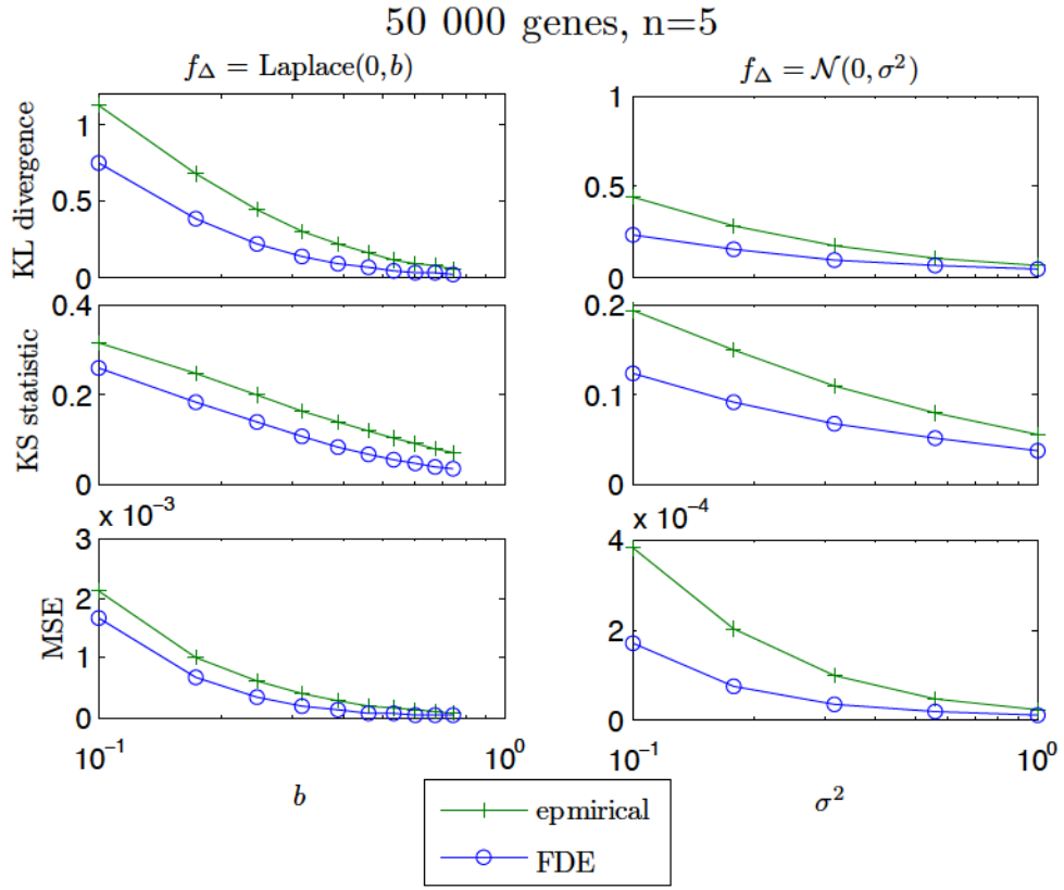
Figure 4.7: Comparison of FDE versus the empirical estimator over the class of zero mean Laplace distributions, and the class of zero mean normal distributions.
